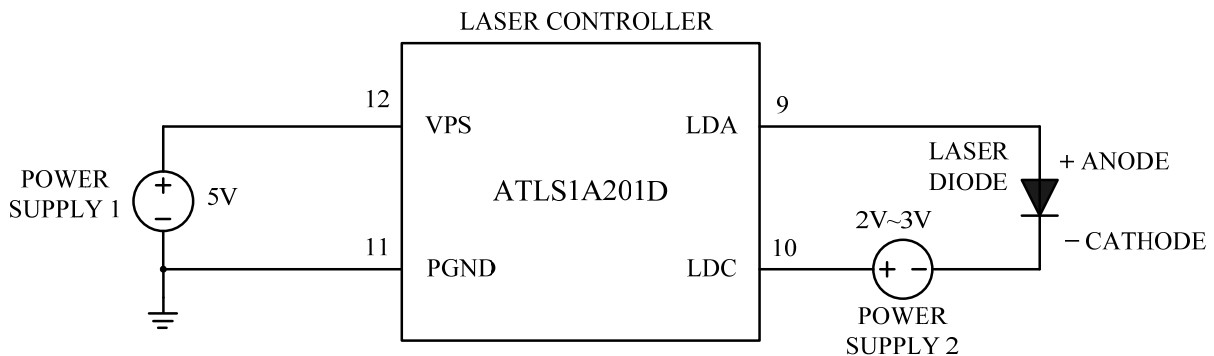
Figure 7. Driving High Voltage Laser Diodes
