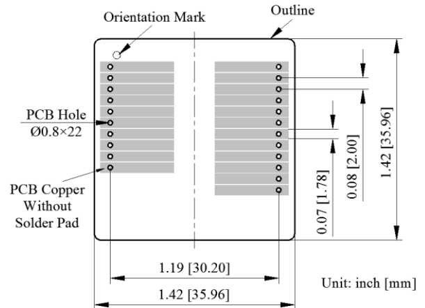
Figure 21. Top View of the Top Side PCB Foot-print
