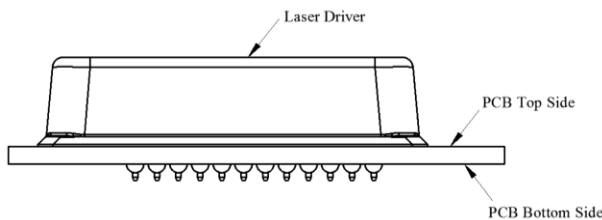
Figure 20. End View of the PCB Foot-print
