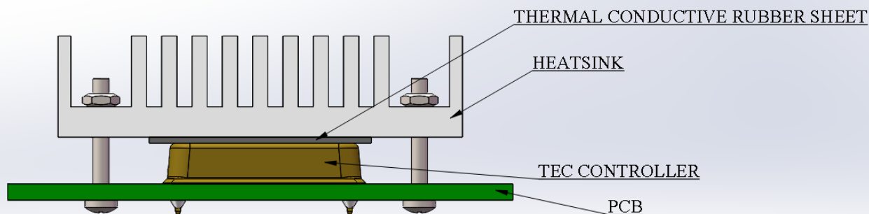
Figure 10.2 Transferring Heat with Heat Sink
