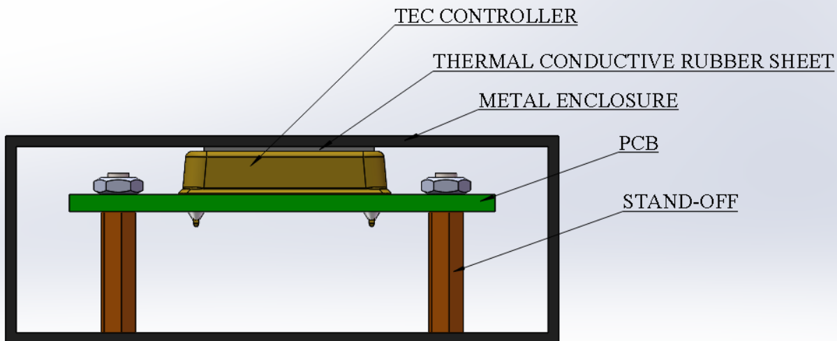
Figure 10.1 Transferring Heat with Metal Enclosure
