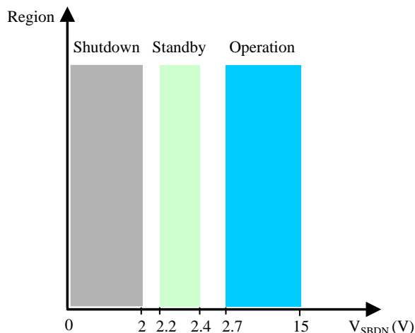
Figure 4. Input Control
