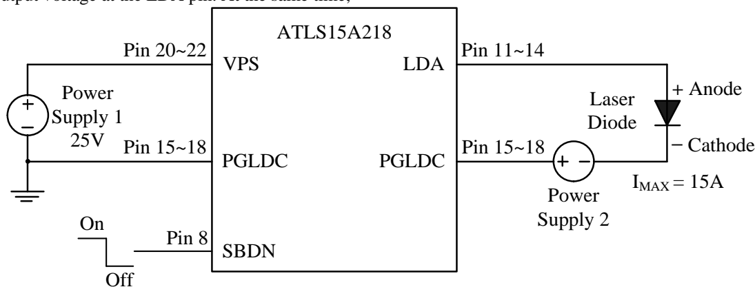
Figure 14. Driving High Voltage Laser Diodes
