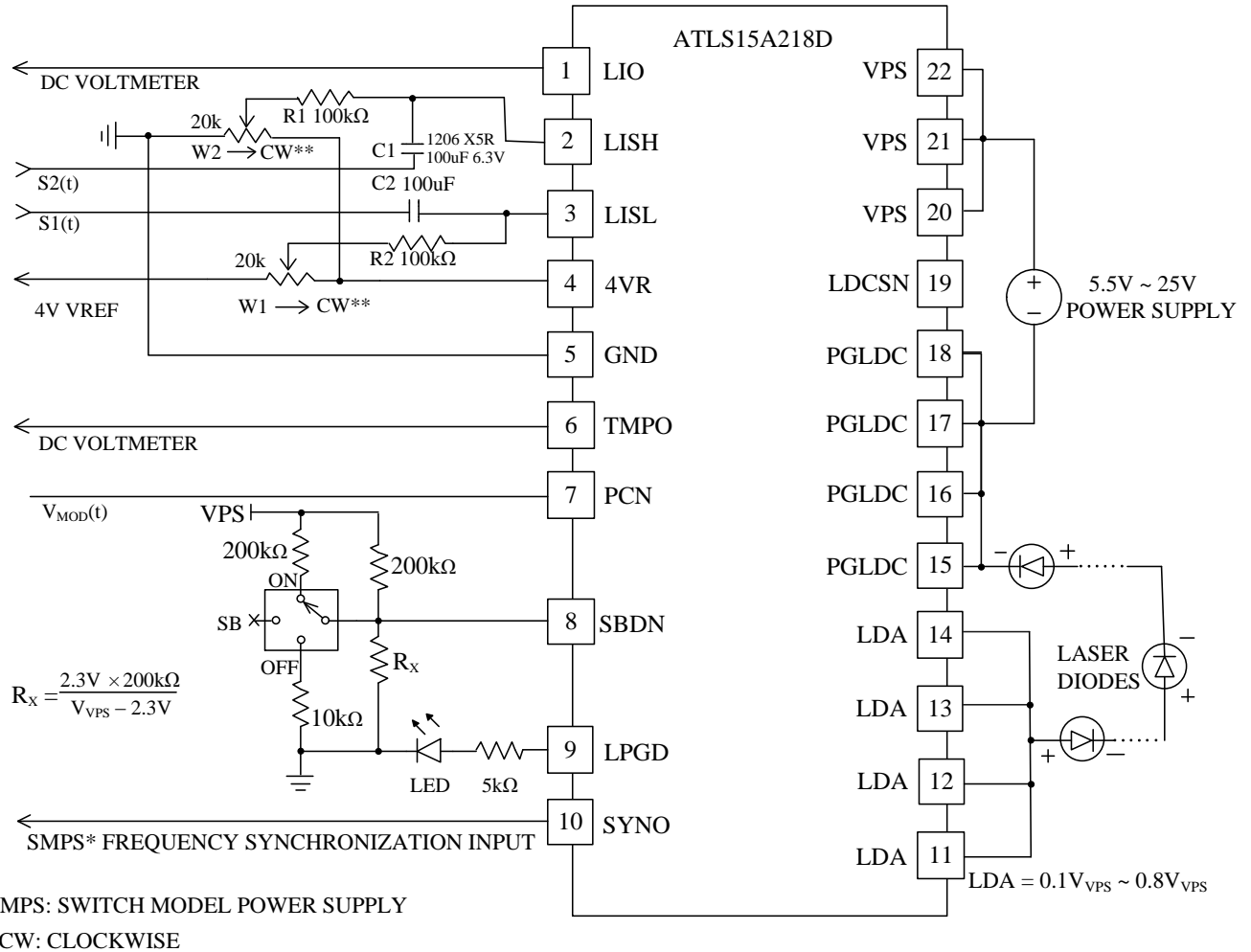
Figure 7. Stand-Alone Application Schematic
