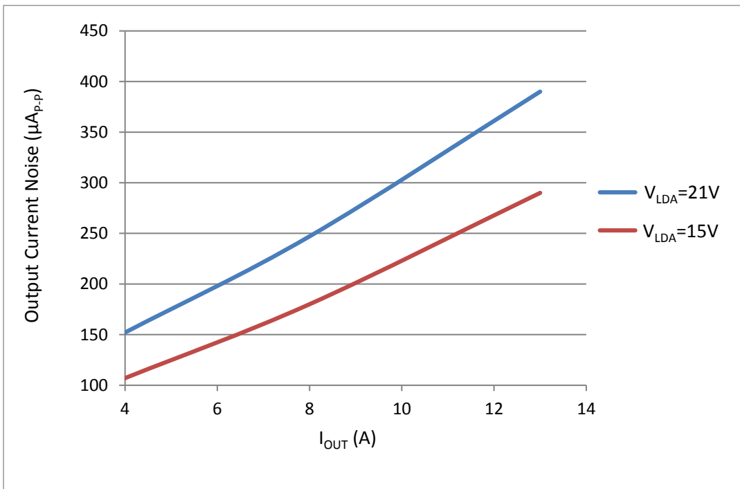
Figure 12. I_{\text{OUT}} vs. Output Current Noise@0.1Hz~10Hz
