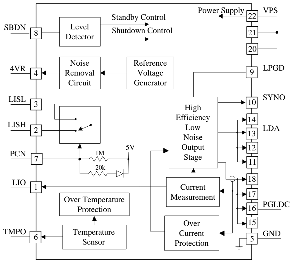
Figure 3. Internal Block Diagram of ATLS15A218
