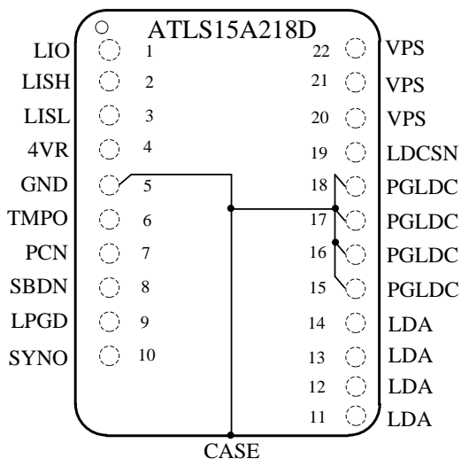
Figure 2. Pin Names and Locations
