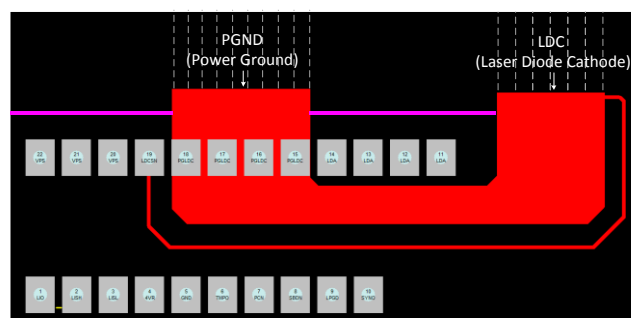
Figure 18. The Layout for the Single-Layer PCB
