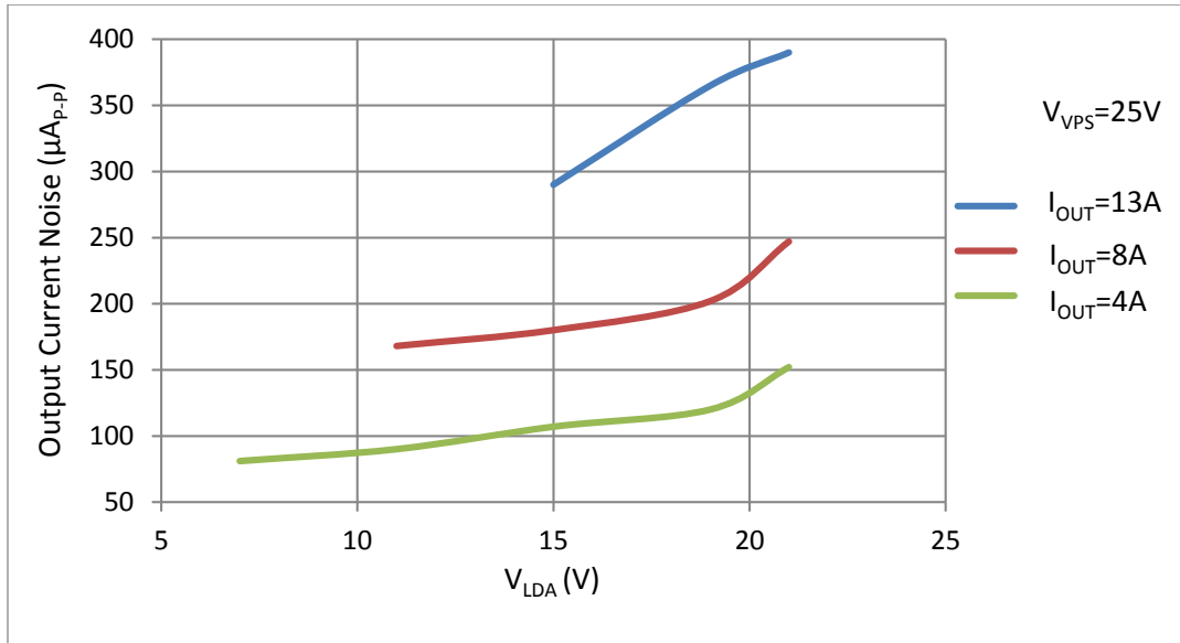
Figure 11. V_{\text{LDA}} vs. Output Current Noise@0.1Hz~10Hz
