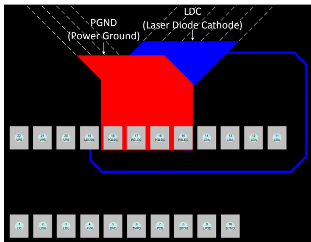
Figure 15. The Layout for the Two-Layer PCB
