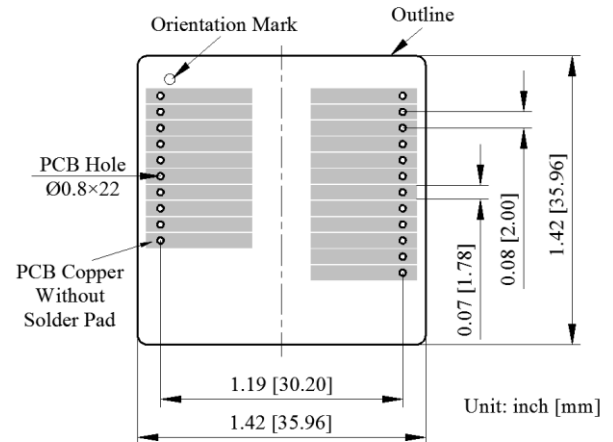
Figure 21. Top View of the Top Side PCB Foot-print
