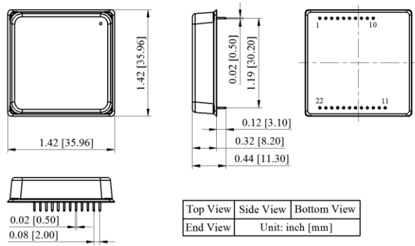
Figure 19. Dimensions of the DIP Package Driver
