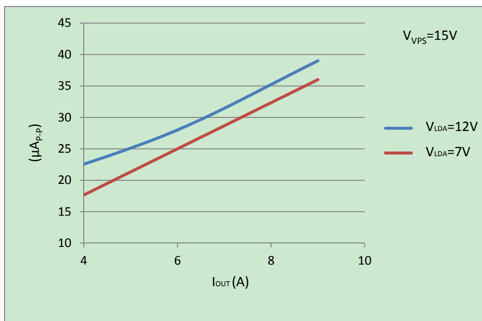
Figure 10.2. I OUT vs. Output Current Noise@0.1Hz~10Hz
