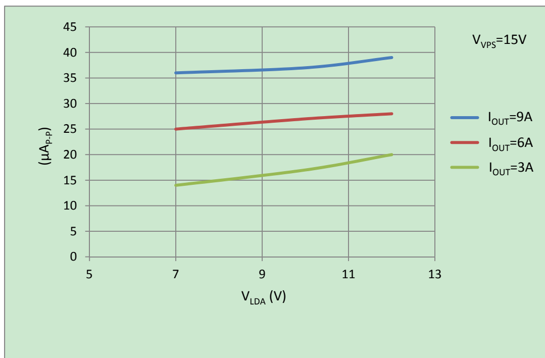
Figure 10.1. V LDA vs. Output Current Noise@0.1Hz~10Hz
