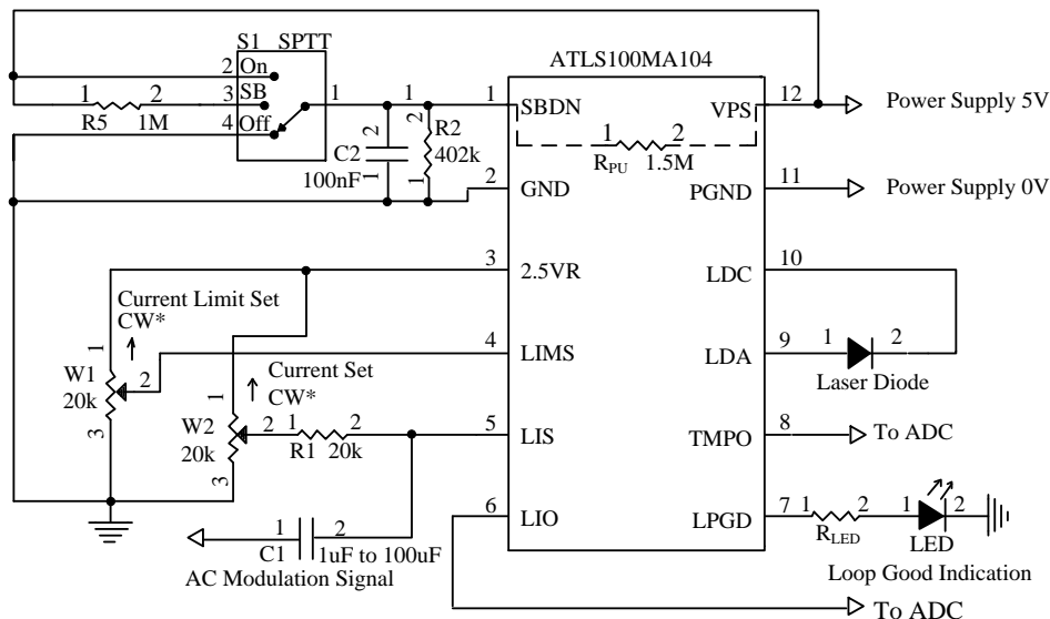
Figure 5.3. Typical AC Modulation with DC bias Schematic for ATLS100MA104
