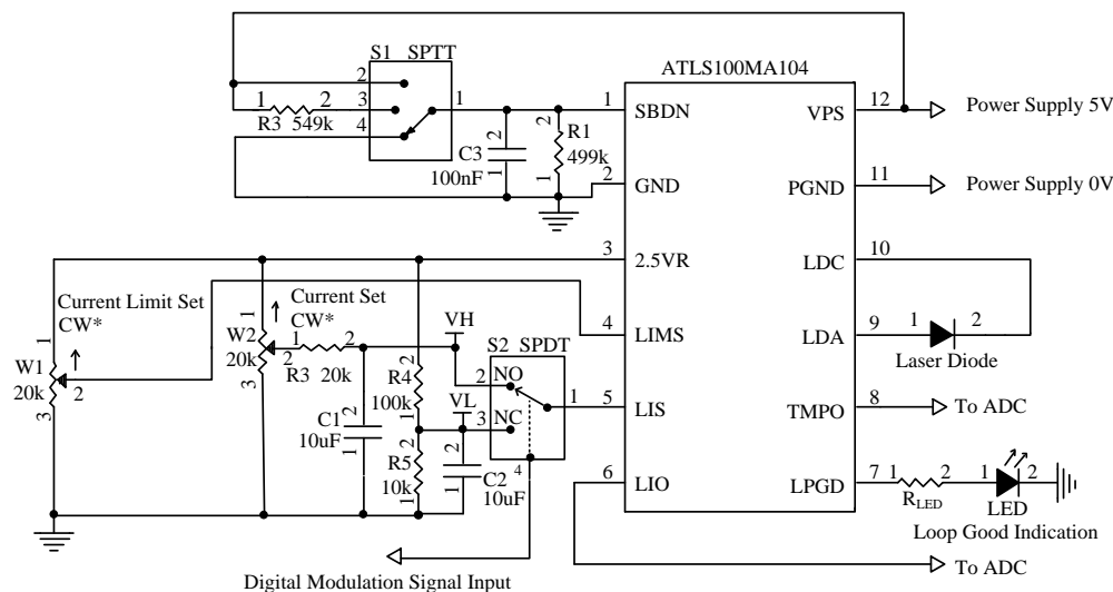
Figure 8. Low Noise Digital Modulation Circuit
