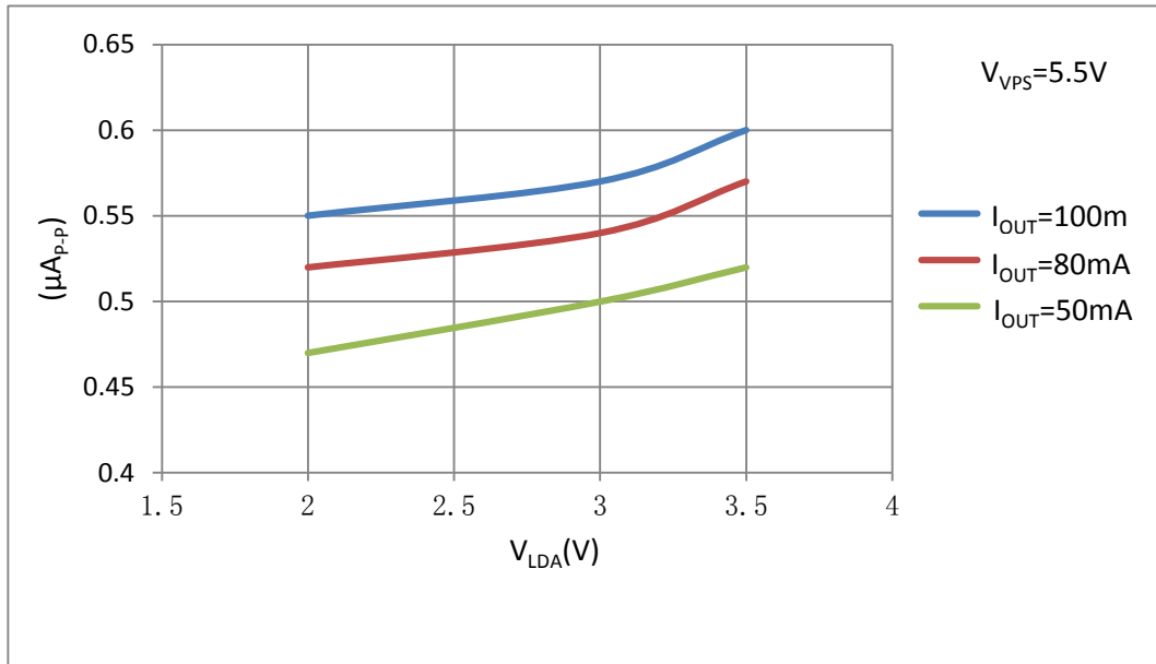
Figure 11.1. V_{LDA} vs. Output Current Noise@0.1Hz~10Hz
