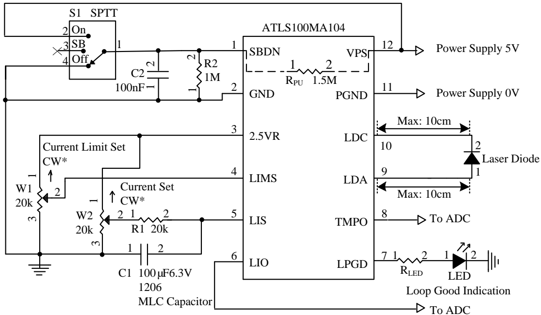
Figure 5.1. Typical Stand-alone CW Operation Schematic for ATLS100MA104
