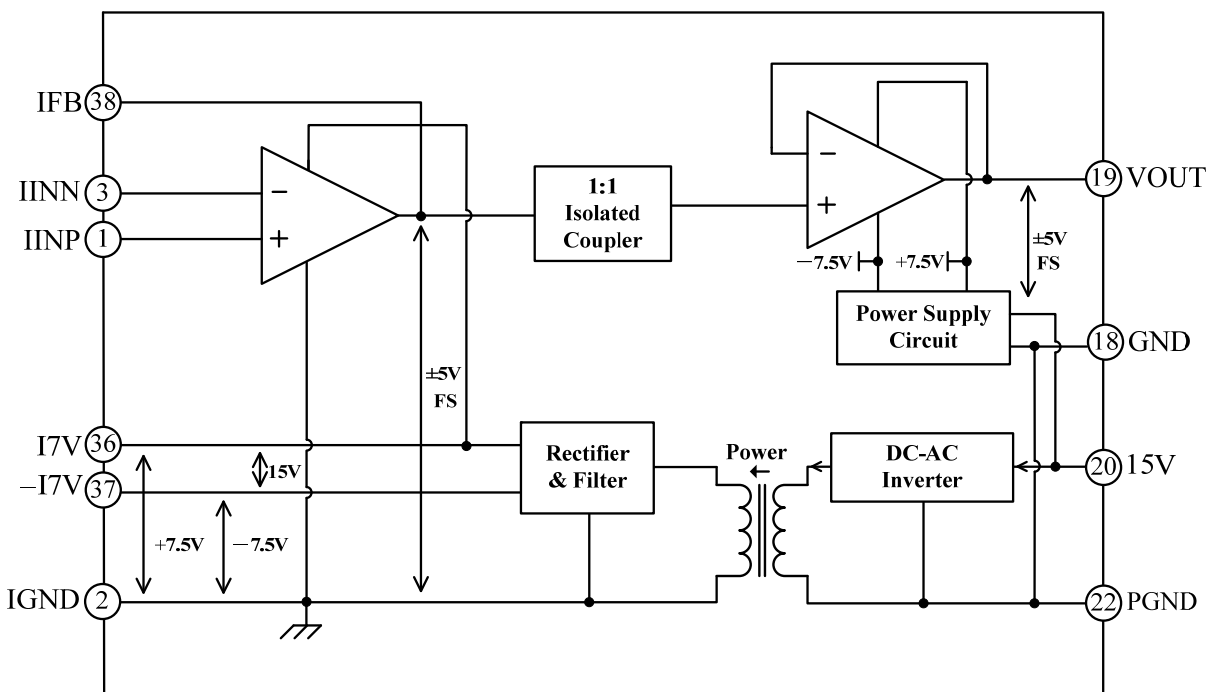
Figure 2. ATIA202KNL Functional Block Diagram
