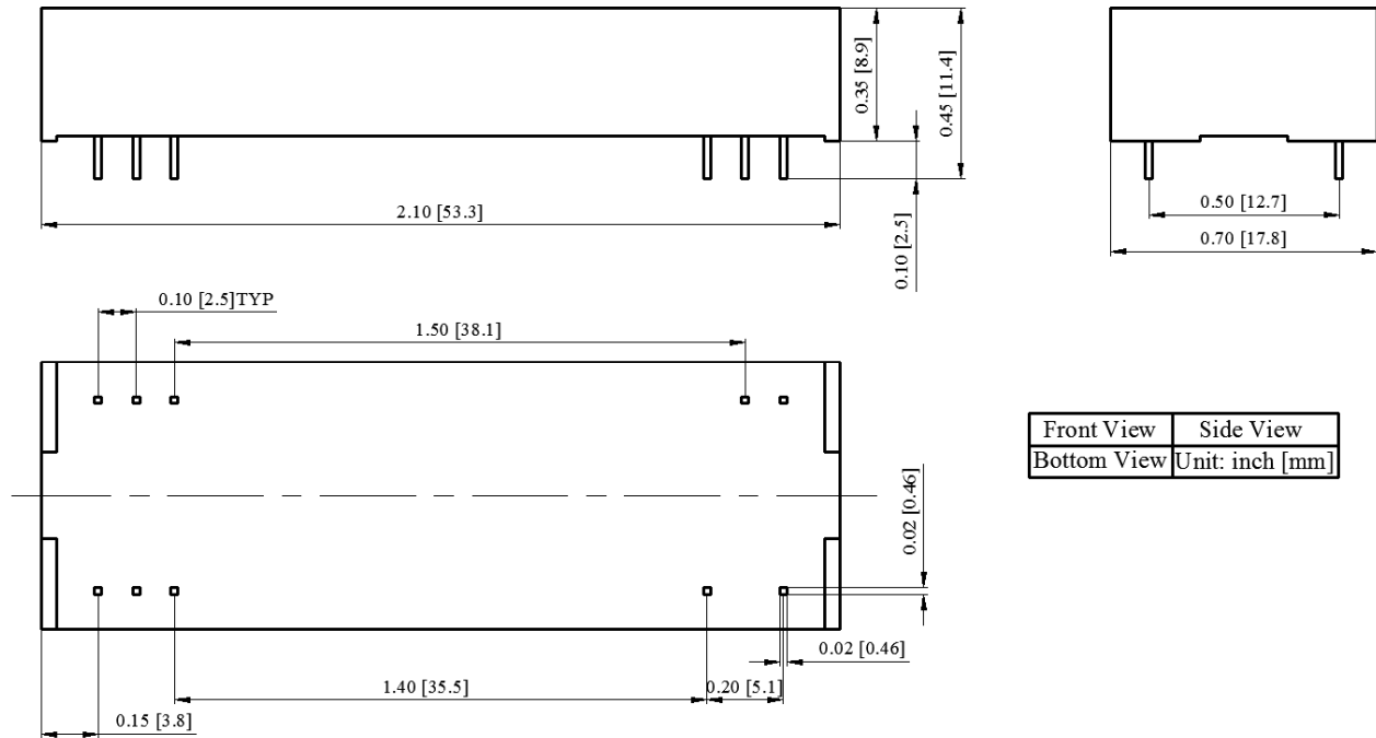
Figure 3. Dimensions of ATIA202KN DIP Package
