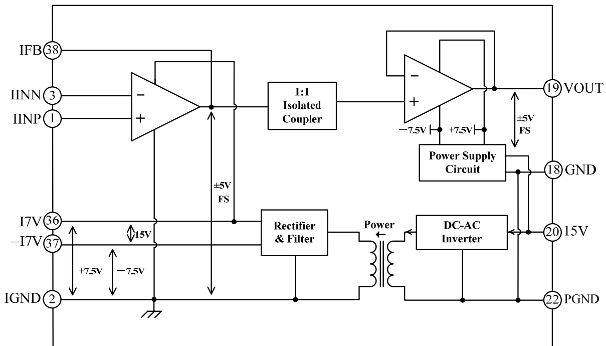
Figure 2. ATIA202JN Functional Block Diagram
