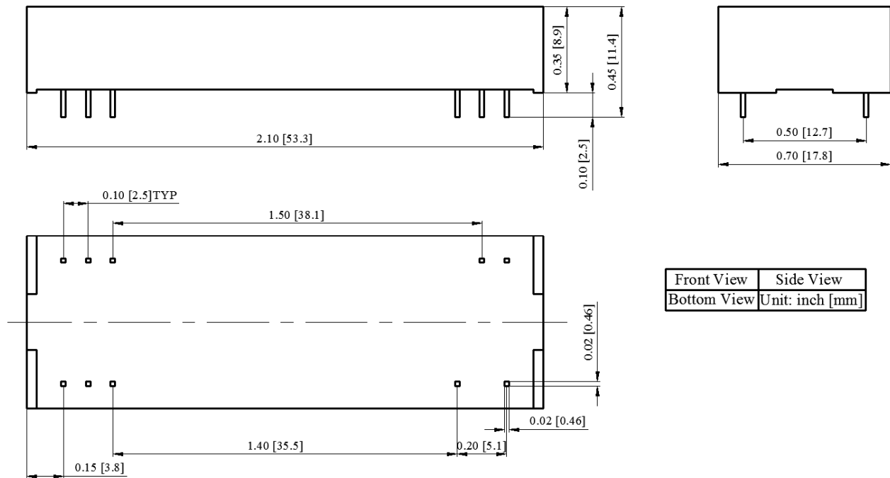
Figure 3. Dimensions of ATIA202JN DIP Package
