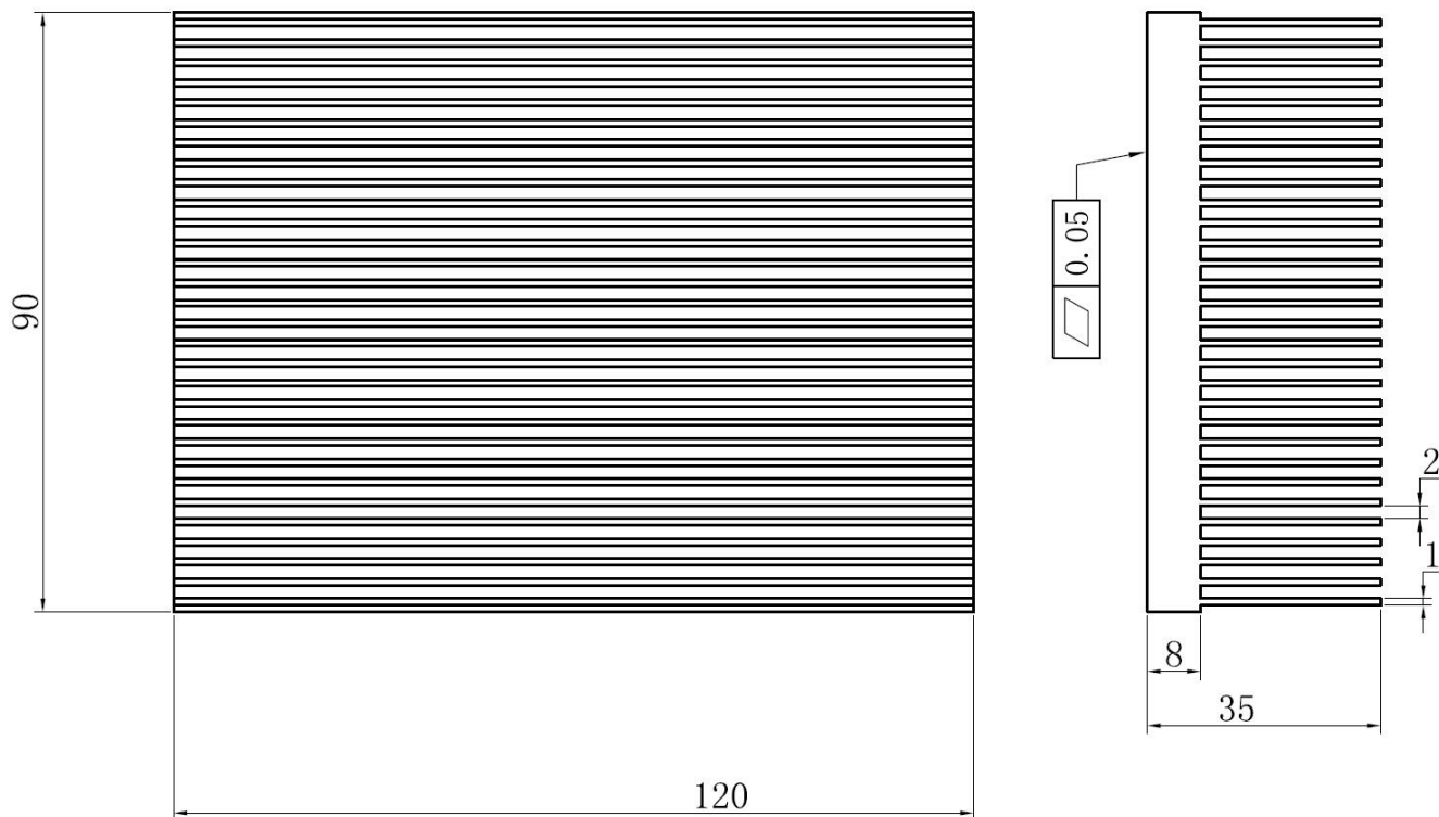
Figure 3. Mechanical Dimensions of Heat Sink ATHS-2/120/90/35A
