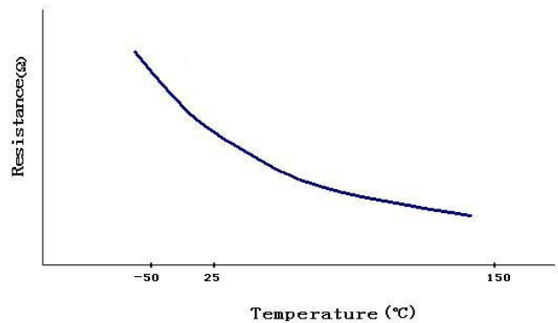
Figure 3. Resistance vs. Temperature for ATH10KHN10
