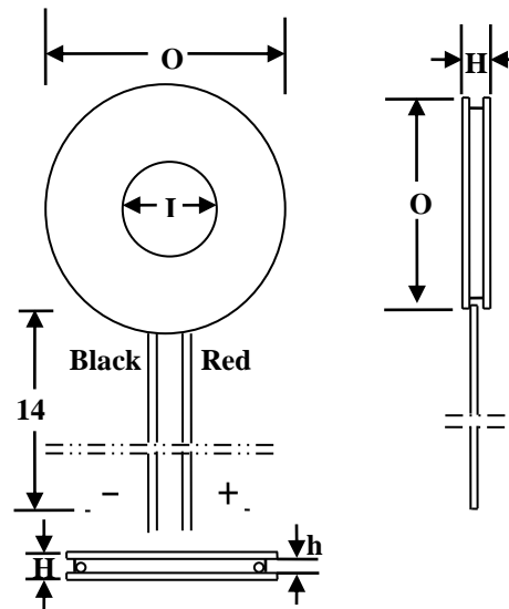
Figure 6. Mechanical Dimensions of ATEC1-38-3.4A
