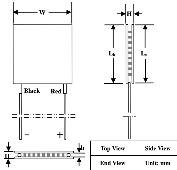
Figure 21. Mechanical Dimensions of Non-sealed ATE1-TCHE-71
