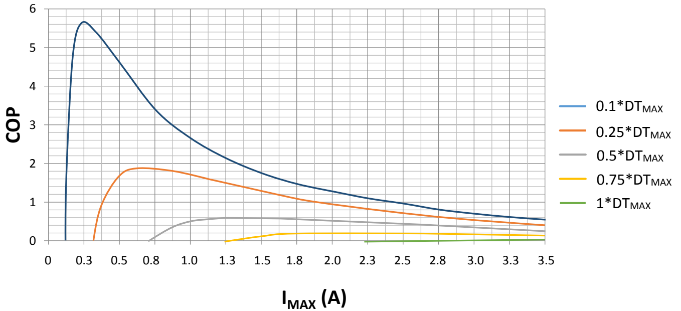
Figure 5. COP vs. I MAX
