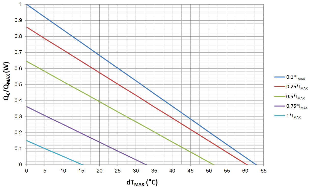
Figure 2. Q_c/Q_{MAX} vs. dT_{MAX}
