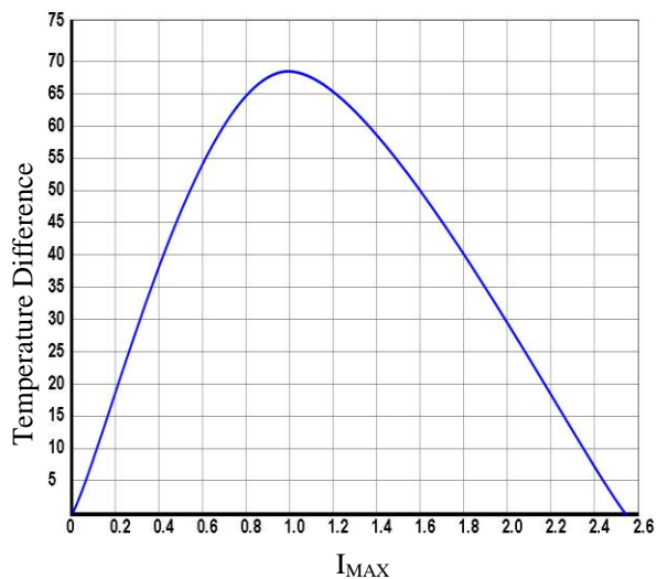
Figure 3. Temperature Difference vs. I_{MAX}
