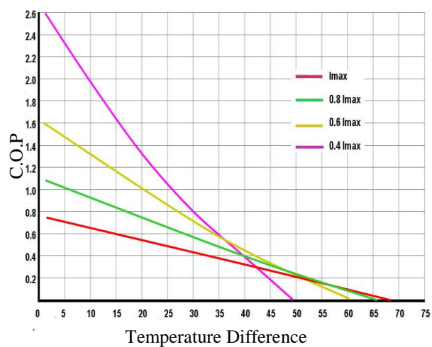
Figure 5. C.O.P vs. Temperature Difference
