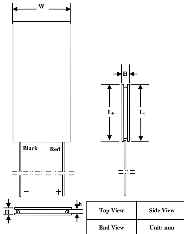
Figure 6. Mechanical Dimensions of ATE1-19
