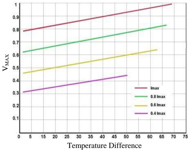
Figure 4. V_{MAX} vs. Temperature Difference
