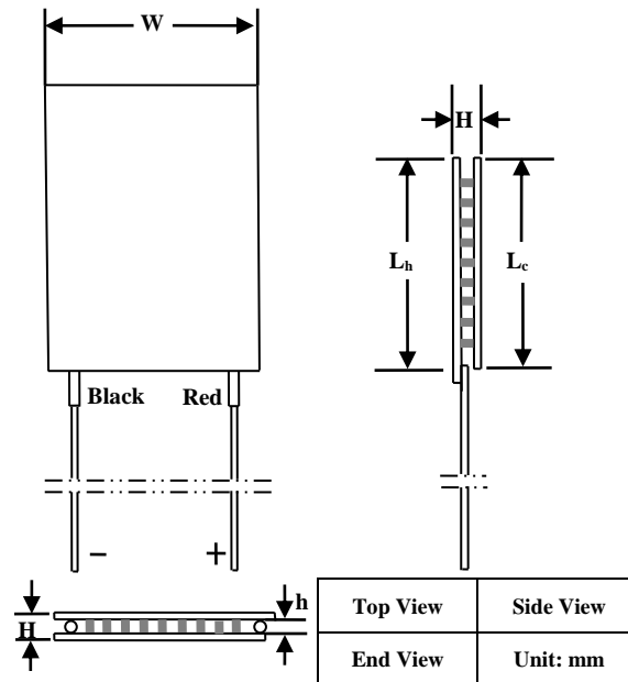
Figure 6. Mechanical Dimensions of Non-sealed ATE1-18
