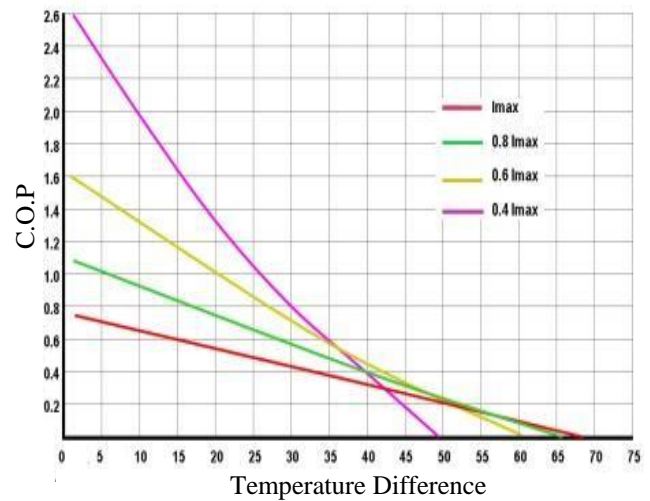
Figure 5. C.O.P vs. Temperature Difference
