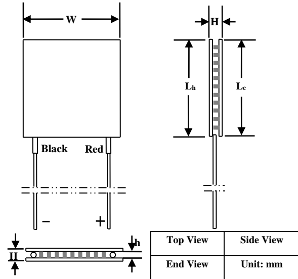
Figure 7. Mechanical Dimensions of Non-sealed ATE1-07
