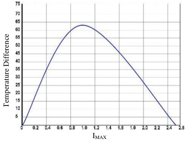
Figure 3. Temperature Difference vs. I MAX
