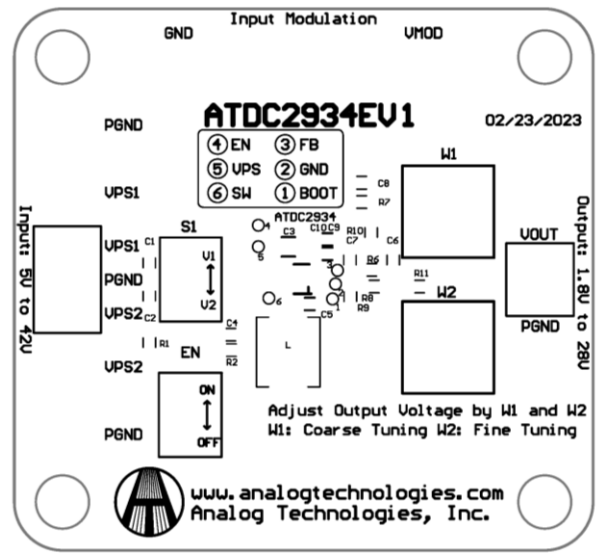
Figure 4. Top Silkscreen
