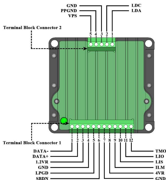
Figure 3. Top View of AQCL3A410SE
