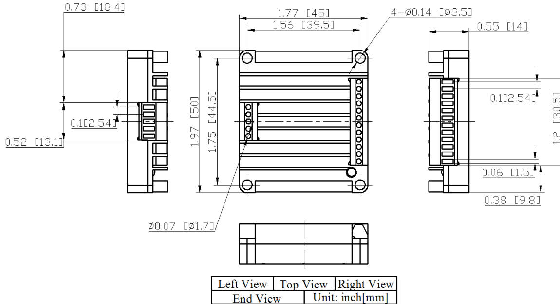
Figure 6. Dimensions of AQCL3A410SE
