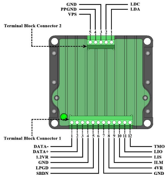
Figure 3. Top View of AQCL2A410SE
