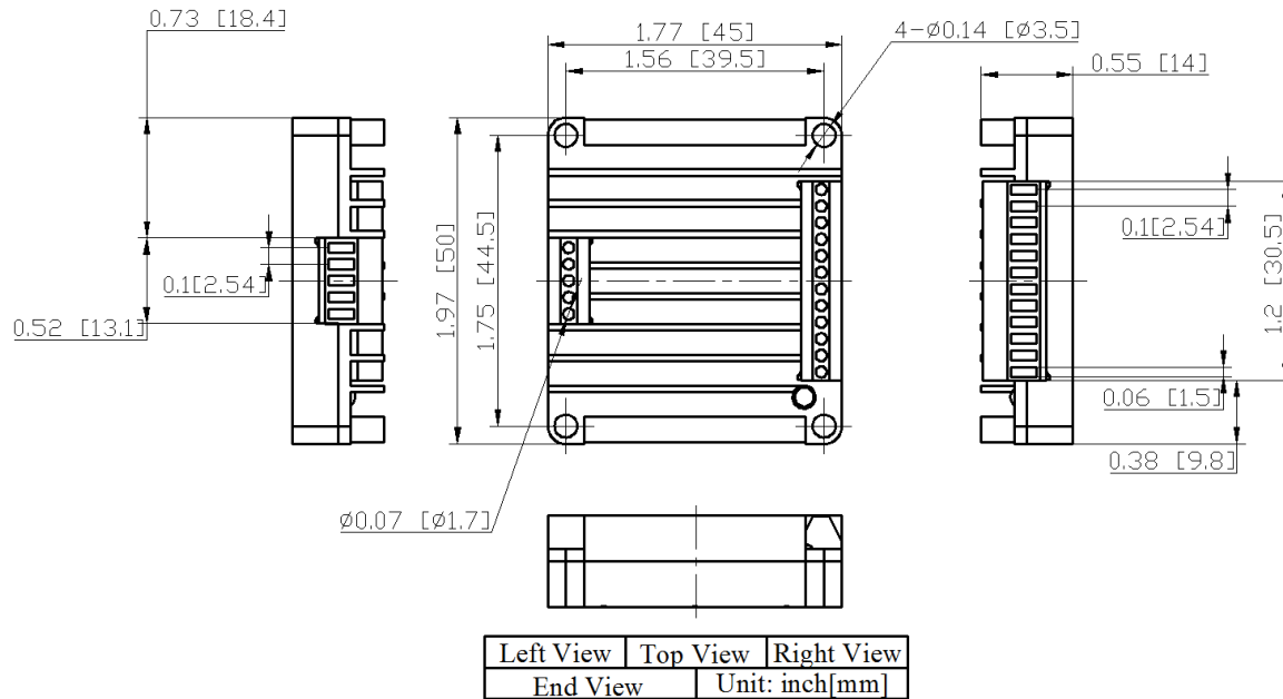
Figure 6. Dimensions of AQCL2A410SE
