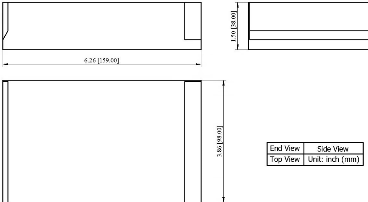
Figure 3. Outline Dimensions
