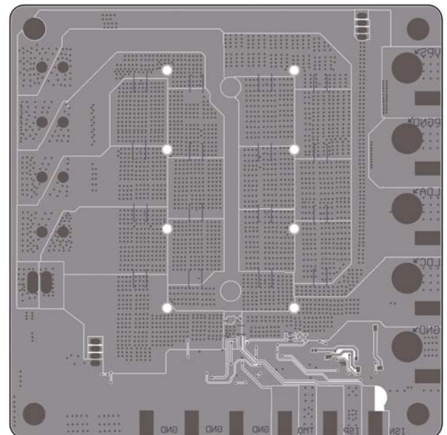
Figure 9. Mirrored Bottom Layers
