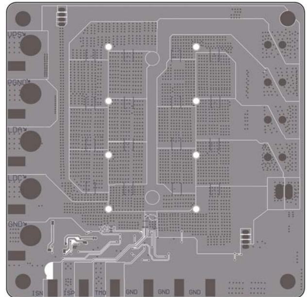
Figure 8. Bottom Layers
