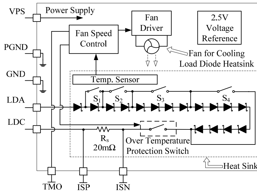
Figure 11. Internal Block Diagram of ALLD10A14V
