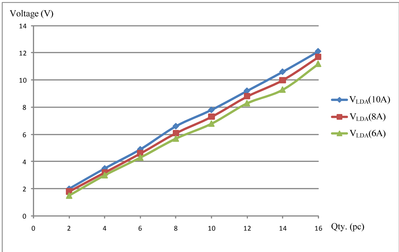
Figure 5. The Voltage of LDA vs. the Quantity of Laser Diodes@ T A =25°C
