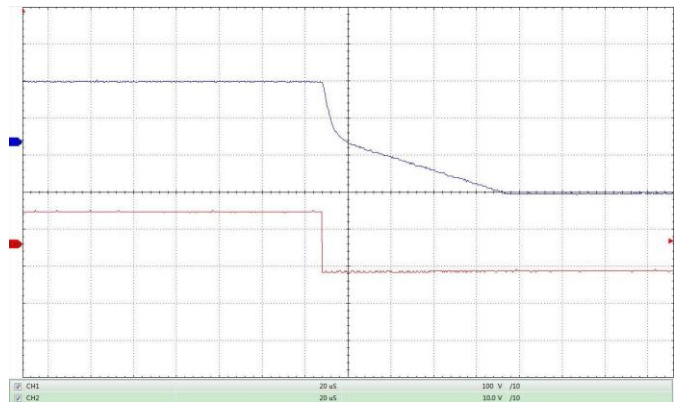
Figure 25. Fall Time
