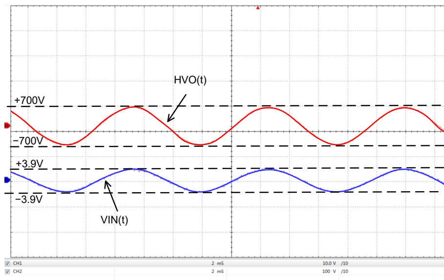
Figure 31. Input vs. Output with Sine Wave
