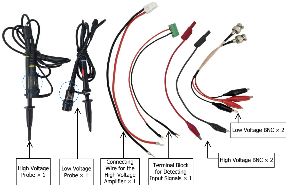
Figure 34. Accessories for the AHVAPN1800V20MABN
