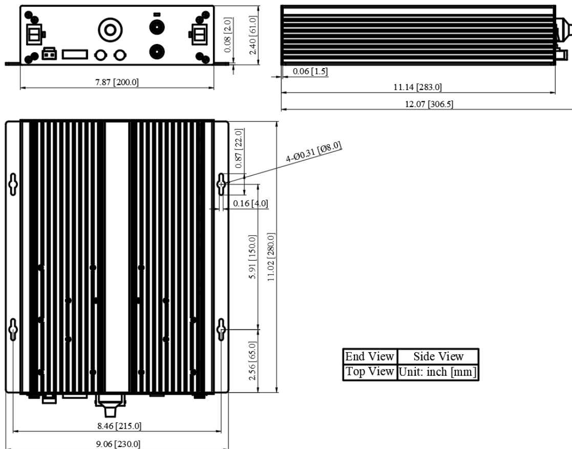
Figure 33. Dimensions of AHVAPN1800V20MABN
