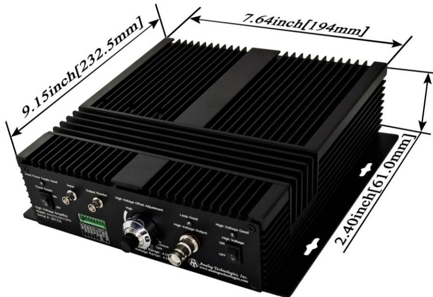
Figure 1A. 3D View
