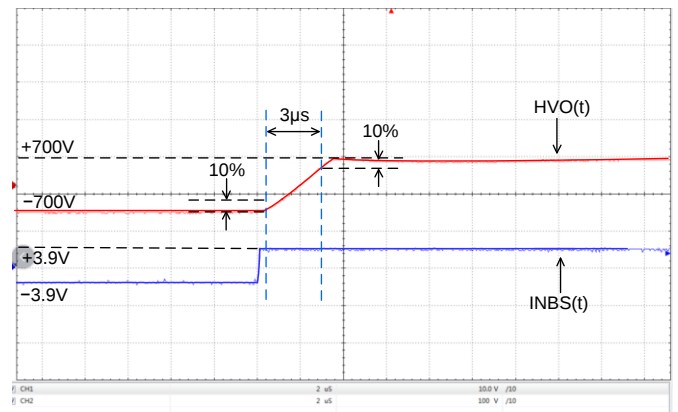
Figure 9. Input vs. Output = \pm 700\text{V} @ 250pF Load
