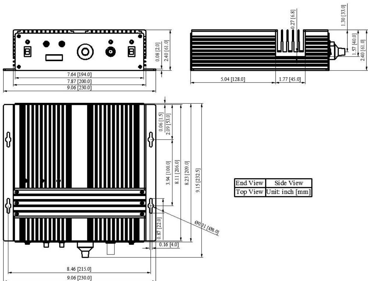
Figure 12. Dimensions of AHVAPN1800V10MA
