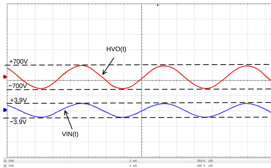
Figure 10. Input vs. Output with Sine Wave
