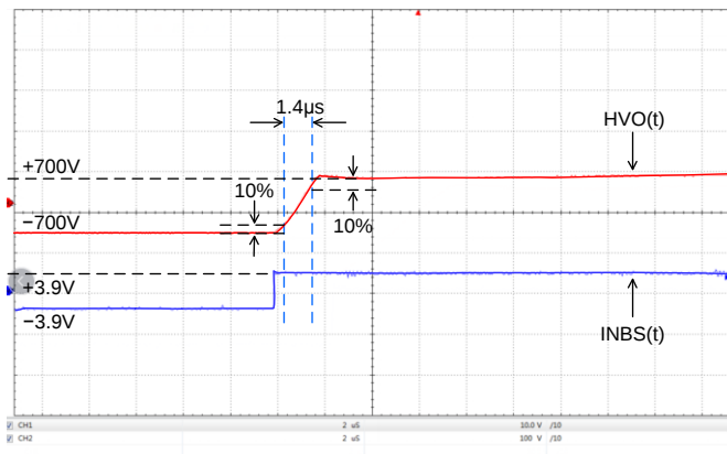
Figure 8. Input vs. Output = \pm 700\text{V} without Load
