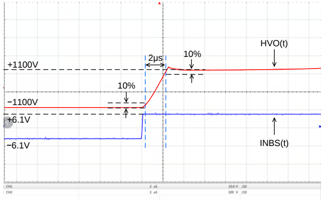
Figure 6. Input vs. Output = \pm 1000\text{V} without Load
