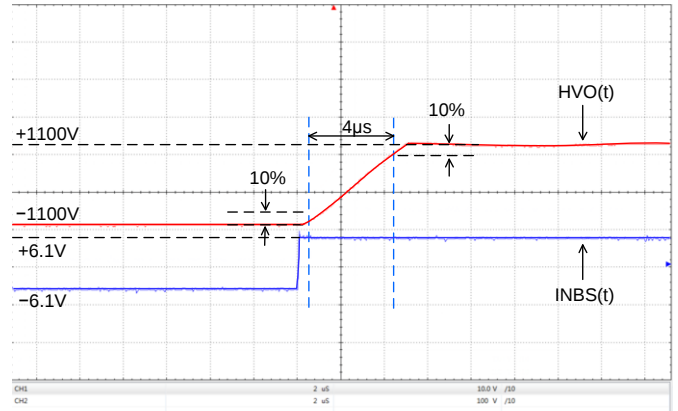
Figure 7. Input vs. Output = \pm 1000\text{V} @ 250pF Load
