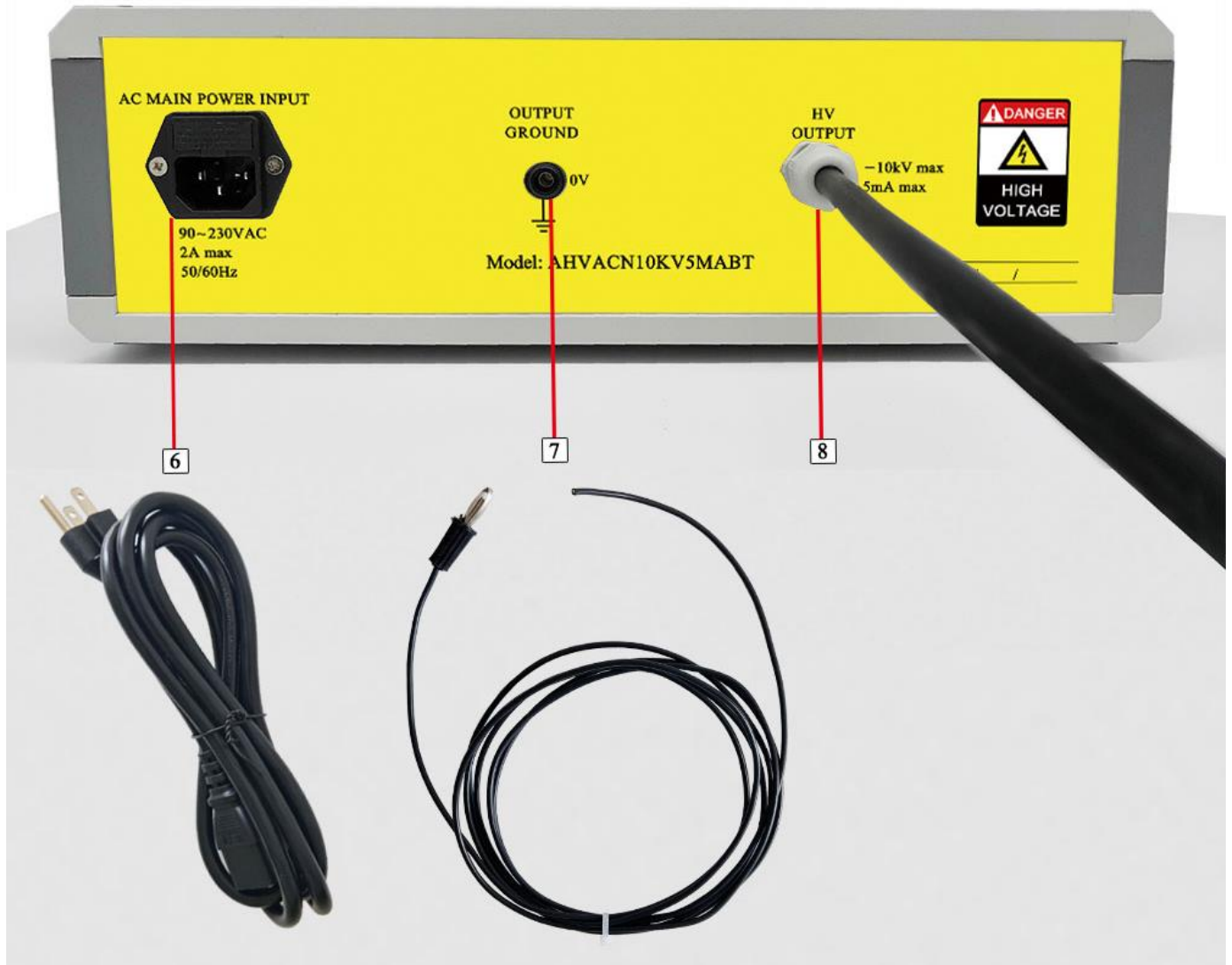
Figure 3. Back Panel
