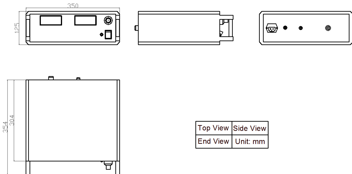
Figure 7. Dimensions for AHVACN10KV10MABT
