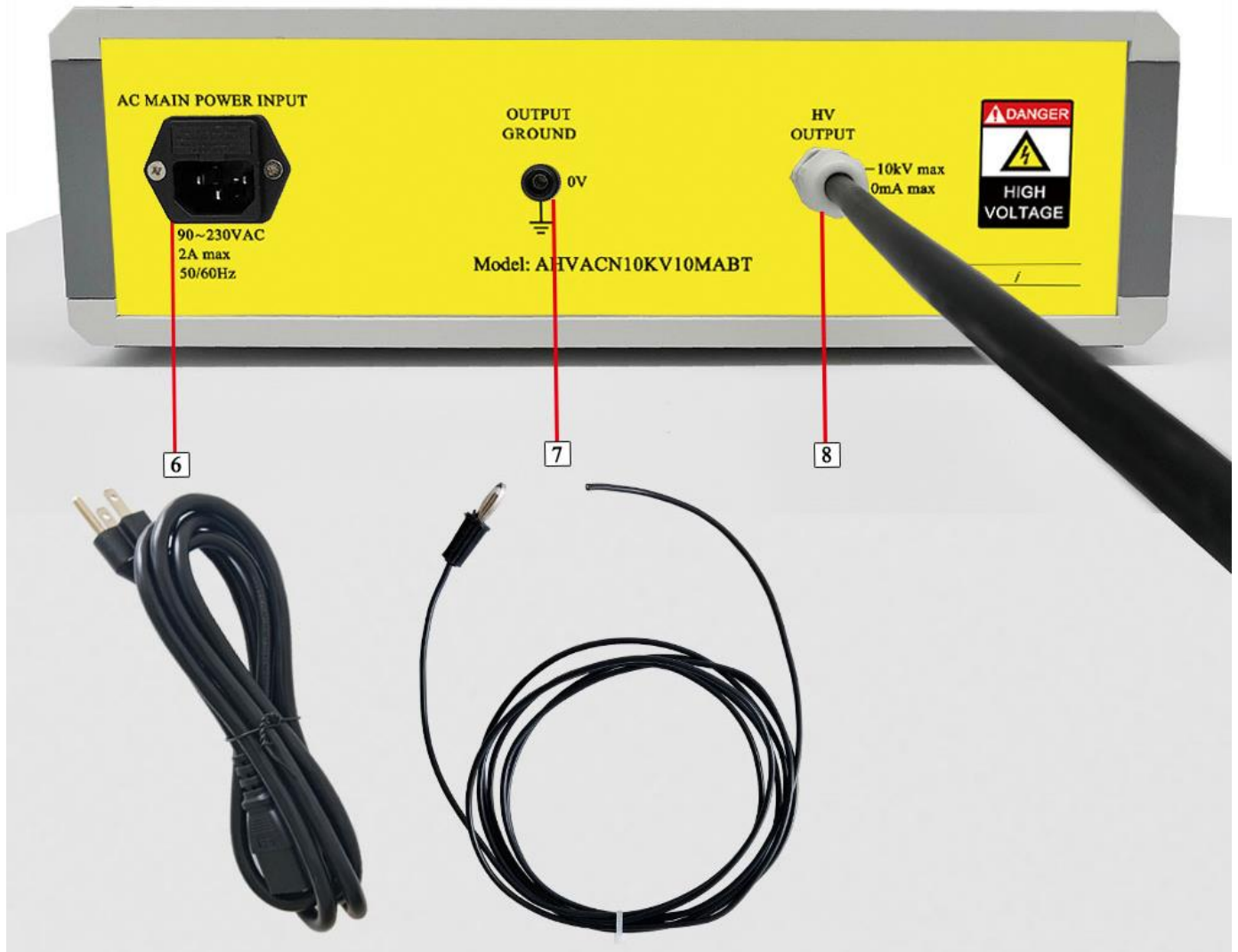
Figure 3. Back Panel
