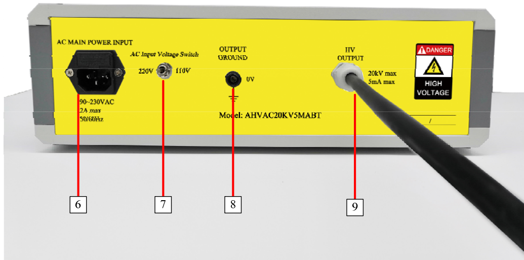
Figure 3. Front Panel
