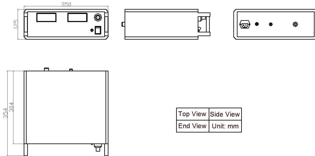
Figure 7. Dimensions for AHVAC20KV1R5MABT
