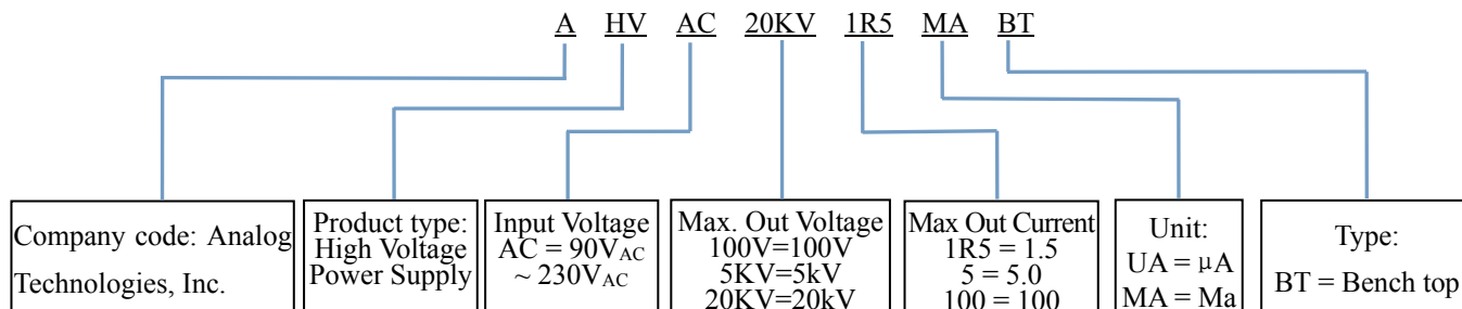
Figure 5. Naming Rules of AHVAC20KV1R5MABT
