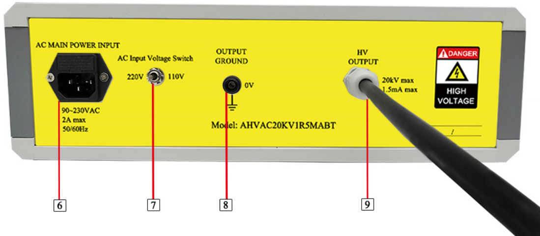
Figure 3. Front Panel
