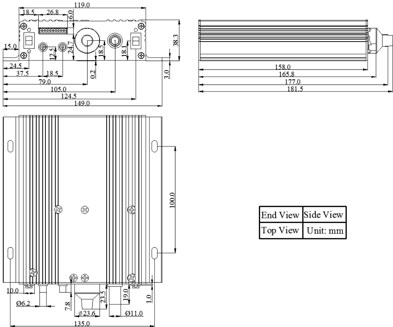
Figure 13. Dimensions of AHVA2KV2X5MA
