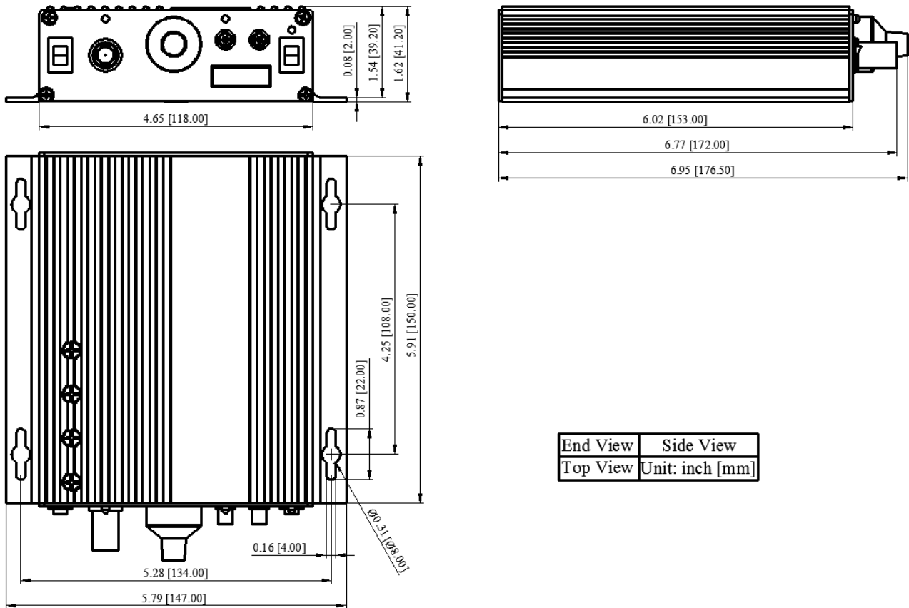
Figure 13. Dimensions of AHVA2KV2X5MA
