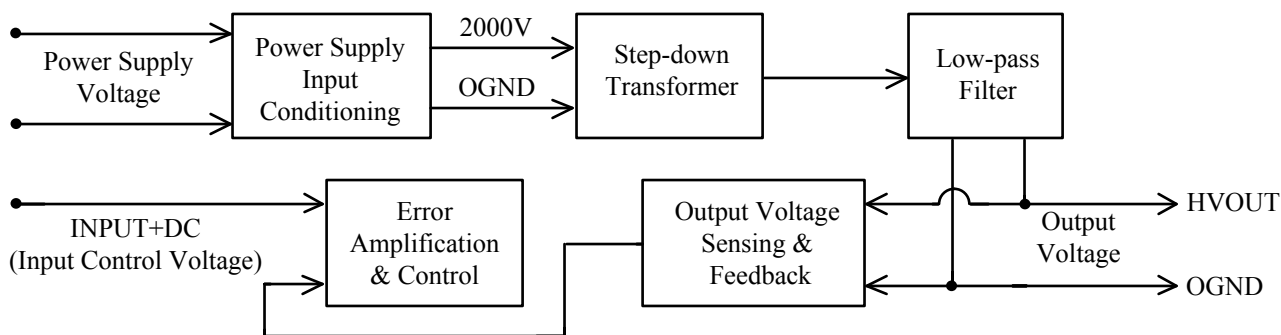
Figure 12. Block Diagram
