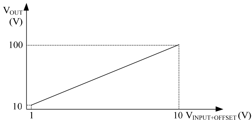
Figure 2. V_{INPUT+OFFSET} vs. V_{OUT}
