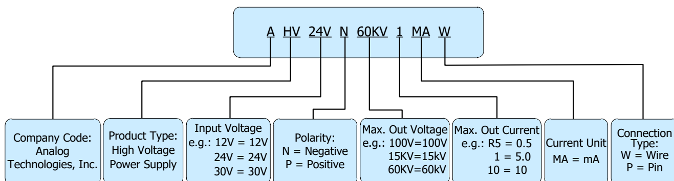
Naming Principle of AHV24VN60KV1MAW
