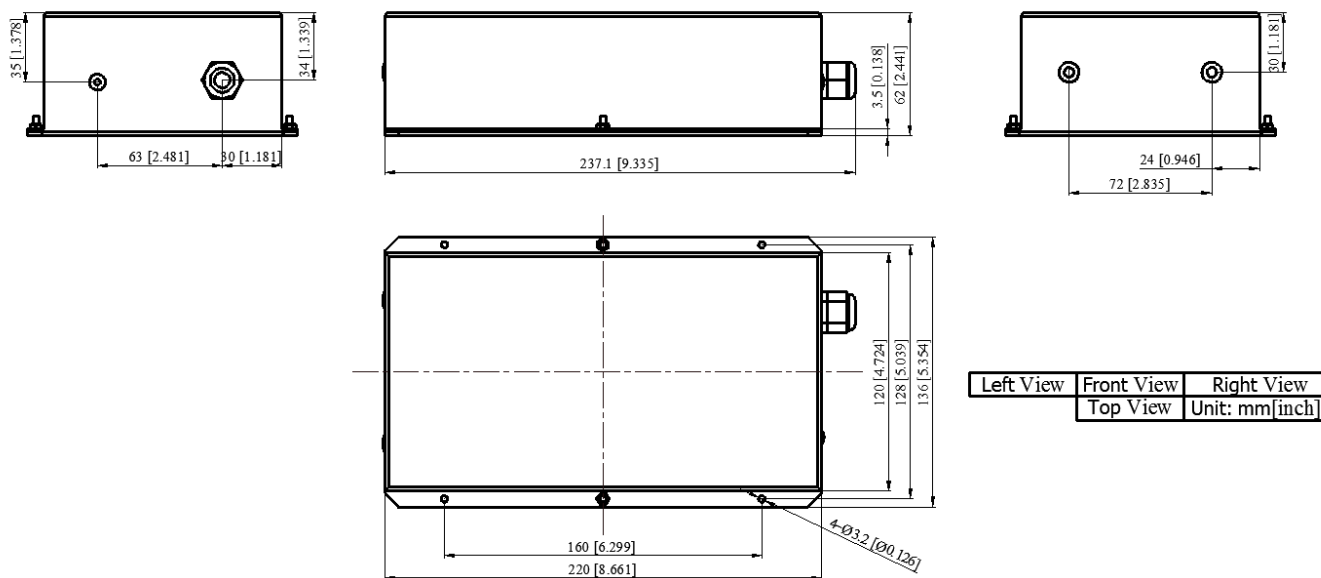
Figure 14. Outline Dimensions
