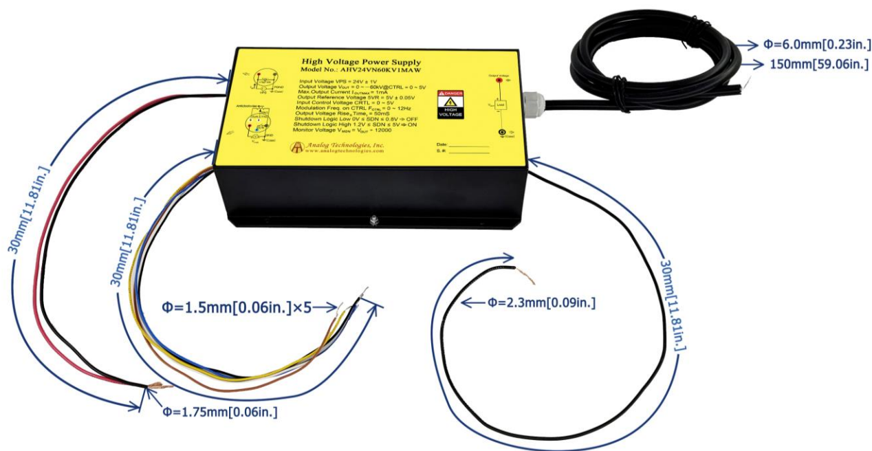
Figure 13. Connecting Lead Wires of AHV24VN60KV1MAW
