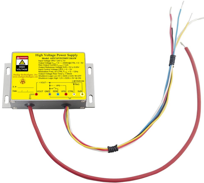
Figure 1.1. Top View of AHV24VN2500V1MAW
