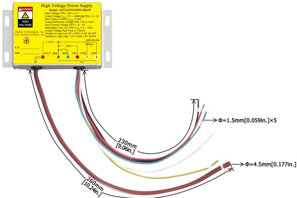
Figure 13. Connecting Lead Wires of AHV24VN2500V1MAW
