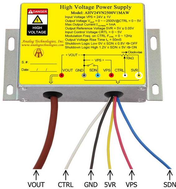
Figure 2. The Connecting Lead Wires of AHV24VN2500V1MAW
