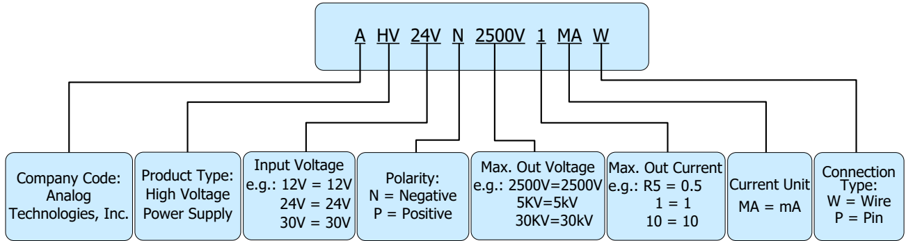
Naming Principle of AHV24VN2500V1MAW
