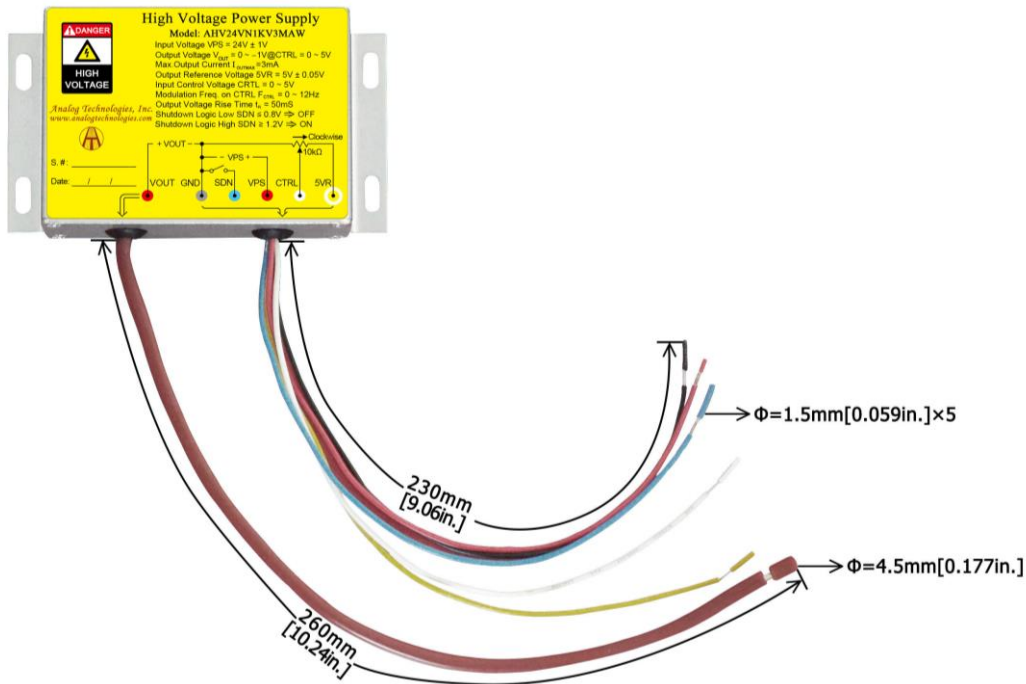
Figure 13. Connecting Lead Wires of AHV24VN1KV3MAW
