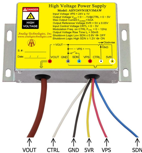
Figure 2. The Connecting Lead Wires of AHV24VN1KV3MAW
