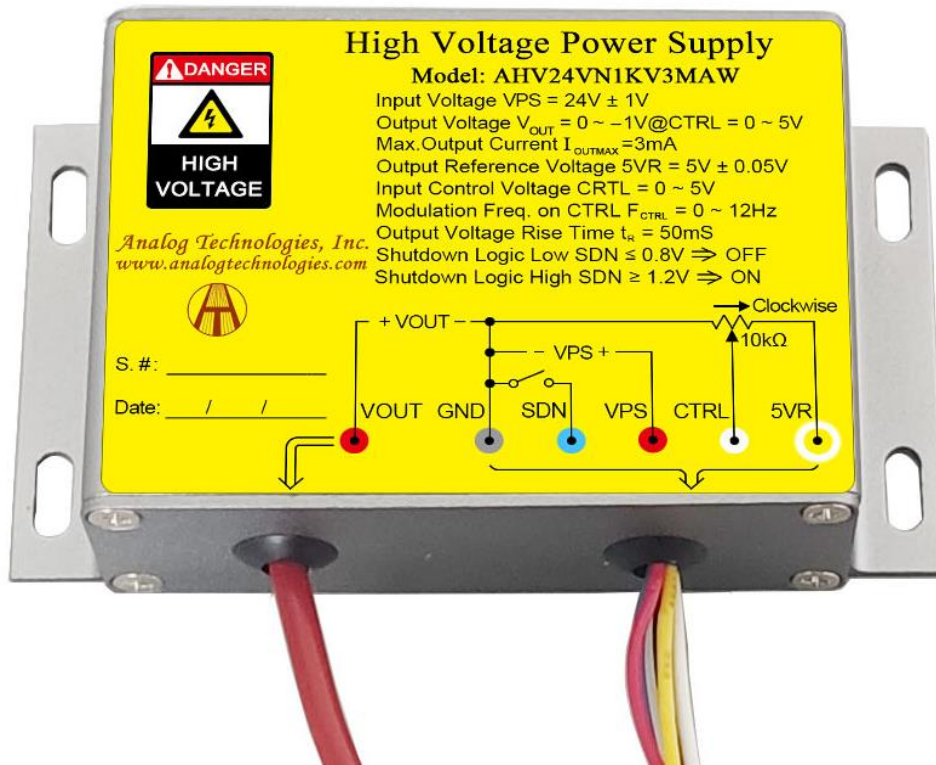
Figure 1.1. Top View of AHV24VN1KV3MAW
