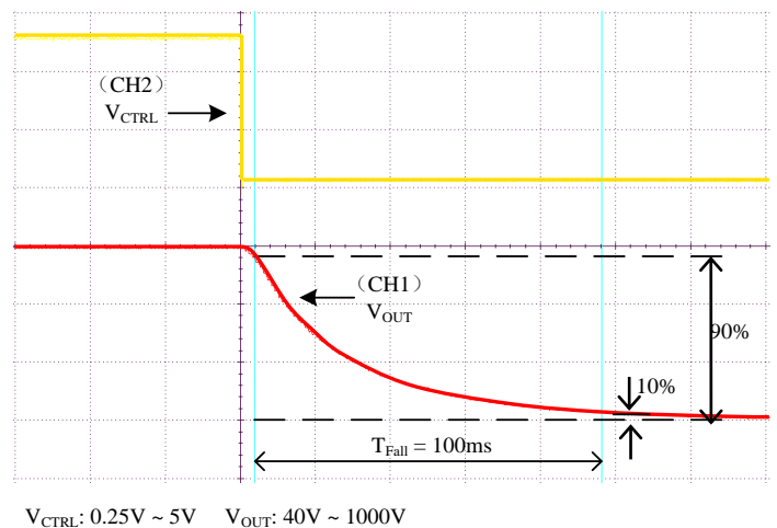
Figure 7. Fall Time
