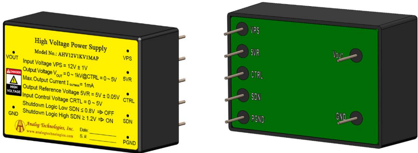
Figure 1. Physical Photo of AHV12V1KV1MAP
