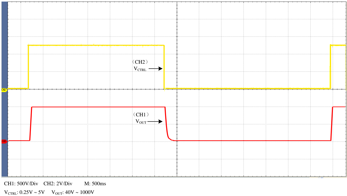
Figure 5. Square Wave
