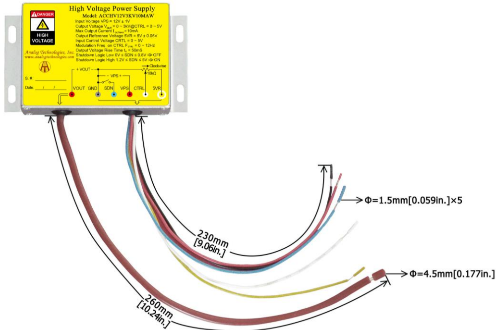
Figure 14. Connecting Lead Wires of ACCHV12V3KV10MAW
