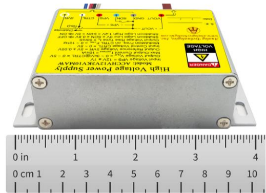
Figure 1.3. Side View
