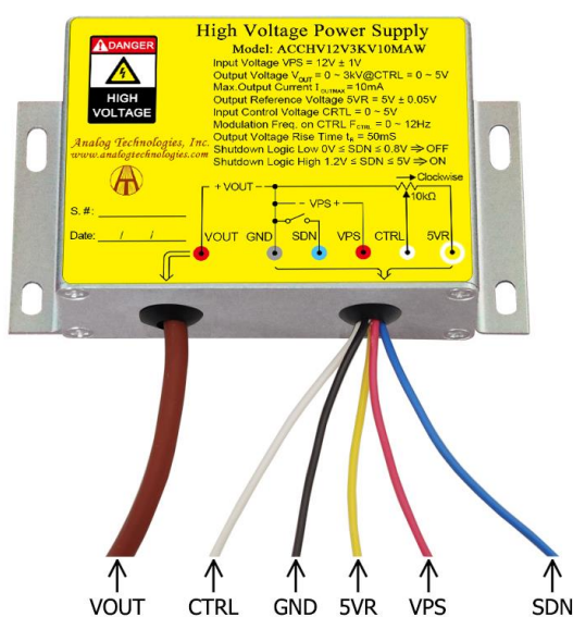
Figure 2. The Connecting Lead Wires of ACCHV12V3KV10MAW
