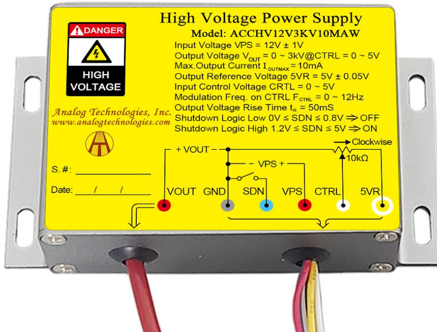
Figure 1.1. Top View of ACCHV12V3KV10MAW
