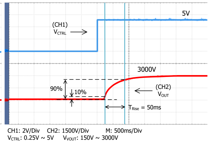
Figure 13. Rising Trail for Large Signal Response
