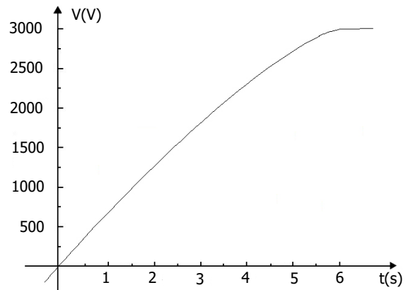
Figure 8. Charging Curve
