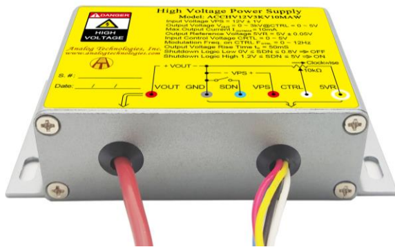
Figure 1.2. Side View
