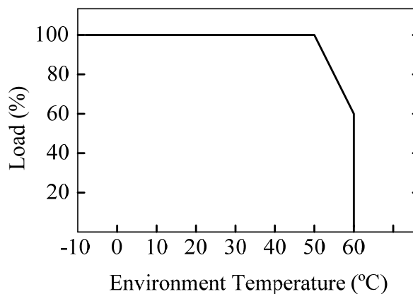
Figure 25. Derating Curve
