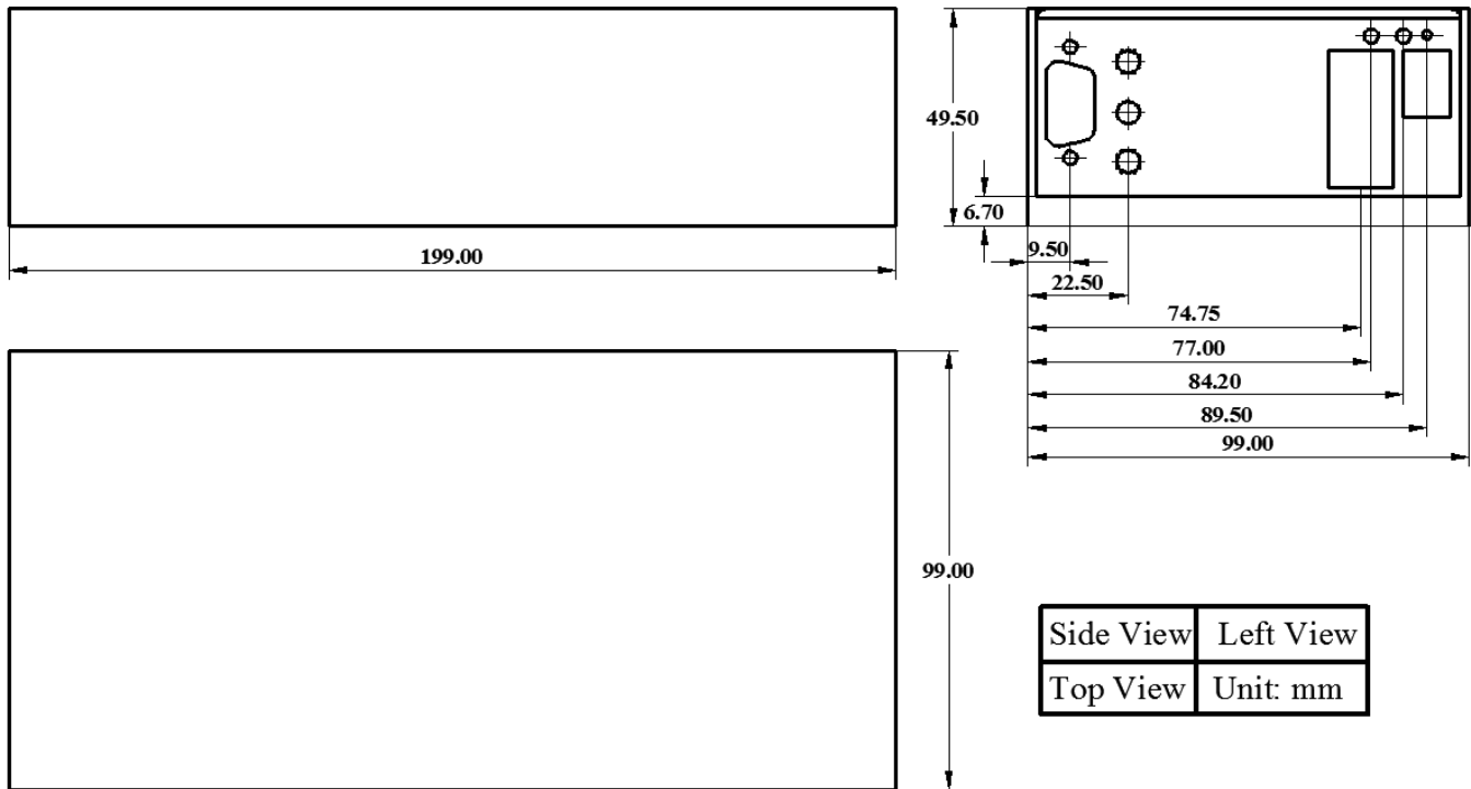
Figure 28. Mechanical Dimensions
