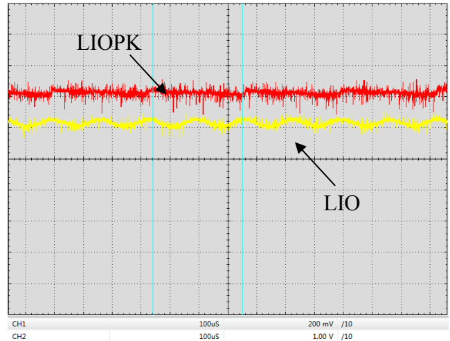
Figure 24. Digital Modulation Response at LIOPK & LIO Pin (f=6kHz)
