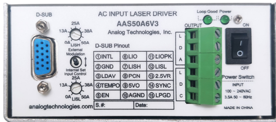
Figure 1. Front View of the AAS50A6V3
