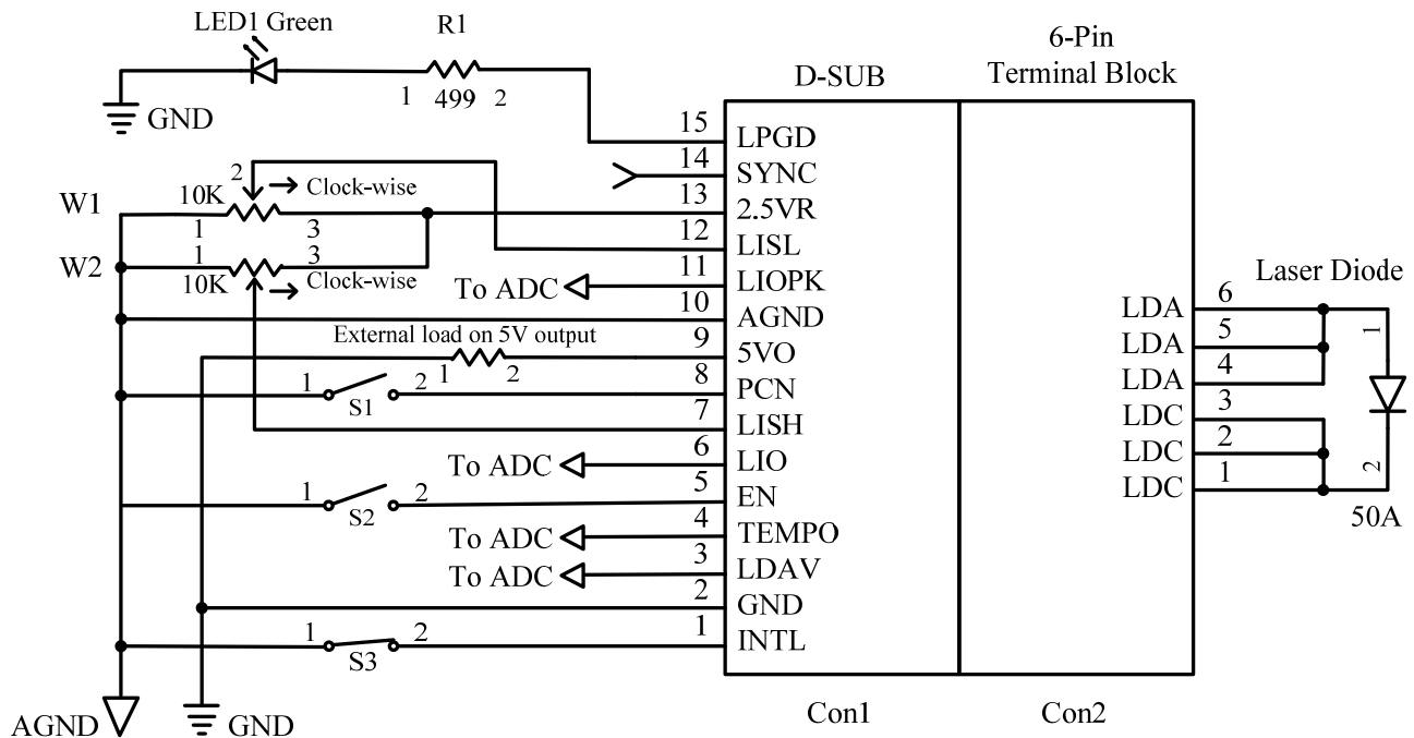
Figure 3. A Typical Application Schematic
