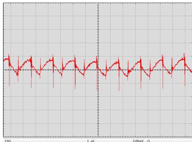
Figure 28. Noise Waveform at LDA Pin
