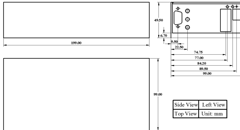
Figure 29. Mechanical Dimensions
