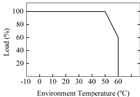
Figure 26. Derating Curve
