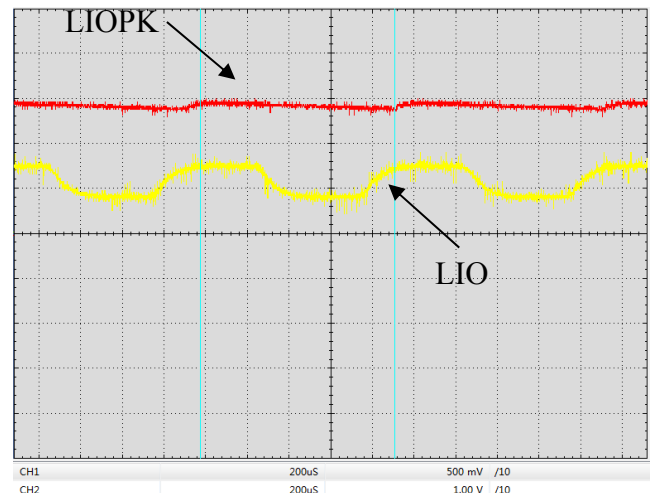
Figure 15. Digital Modulation Response at LIOPK & LIO Pin (f=1kHz)
