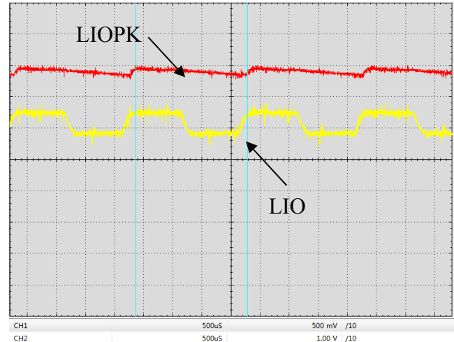
Figure 13. Digital Modulation Response at LIOPK & LIO Pin (f=500Hz)
