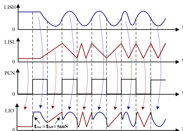
Figure 5. Digitally Controlled Analog Modulation Principle
