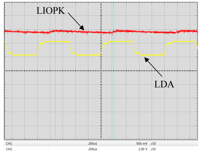
Figure 13. Digital Modulation Response at LIOPK & LDA Pin (f=1kHz)
