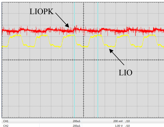
Figure 16. Digital Modulation Response at LIOPK & LIO Pin ( f=2\text{kHz} )
