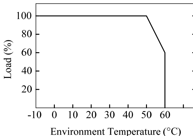
Figure 25. Derating Curve
