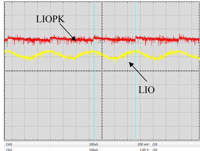
Figure 18. Digital Modulation Response at LIOPK & LIO Pin ( f=3\text{kHz} )
