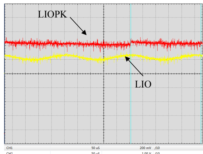
Figure 20. Digital Modulation Response at LIOPK & LIO Pin ( f=4\text{kHz} )
