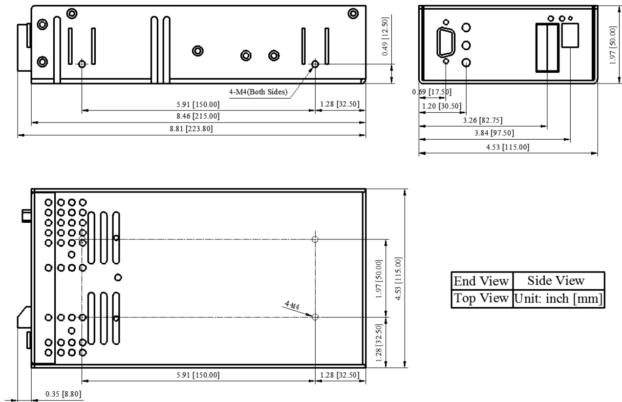
Figure 28. Mechanical Dimensions
