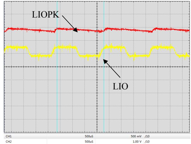
Figure 12. Digital Modulation Response at LIOPK & LIO Pin (f=500Hz)
