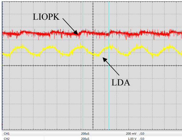
Figure 15. Digital Modulation Response at LIOPK & LDA Pin ( f=2\text{kHz} )
