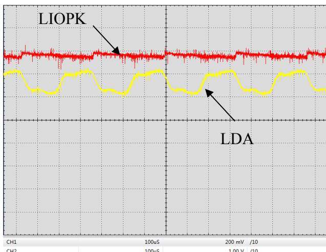
Figure 17. Digital Modulation Response at LIOPK & LDA Pin ( f=3\text{kHz} )
