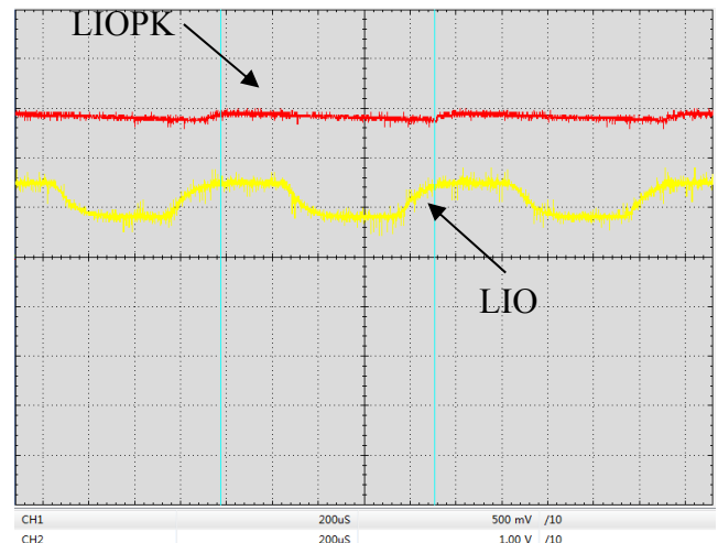
Figure 14. Digital Modulation Response at LIOPK & LIO Pin (f=1kHz)
