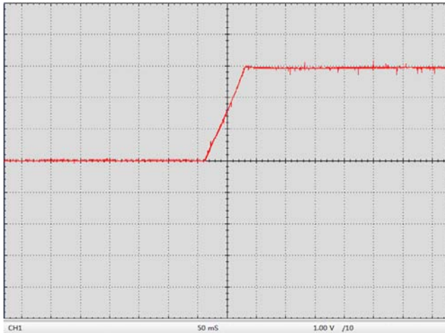
Figure 26. Start-up Waveform at LDA Pin
