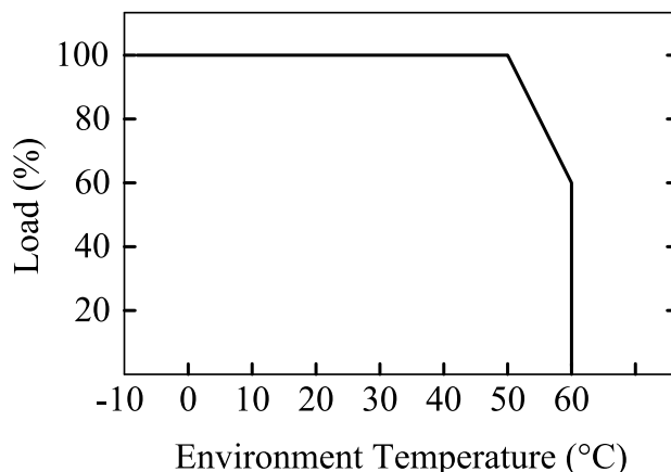
Figure 27. Derating Curve
