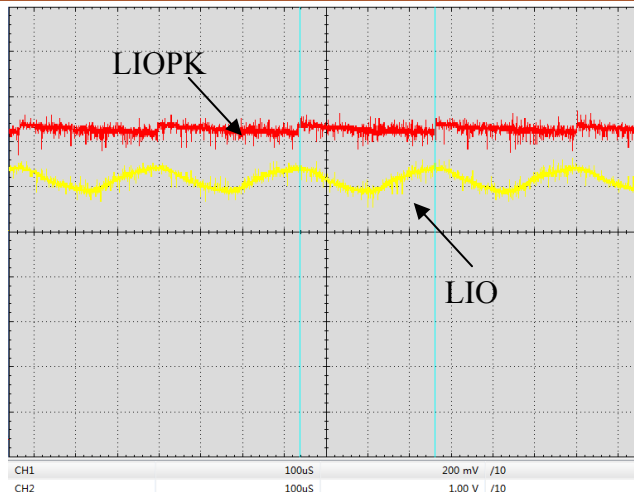
Figure 20. Digital Modulation Response at LIOPK & LIO Pin (f=3kHz)
