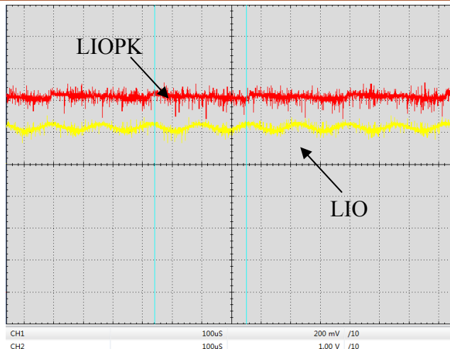
Figure 26. Digital Modulation Response at LIOPK & LIO Pin (f=6kHz)
