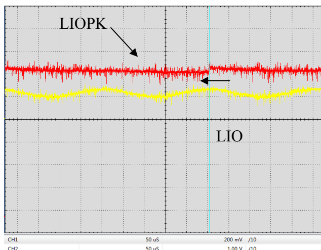
Figure 22. Digital Modulation Response at LIOPK & LIO Pin (f=4kHz)
