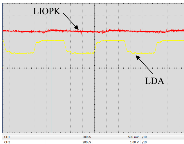
Figure 15. Digital Modulation Response at LIOPK & LDA Pin (f=1kHz)
