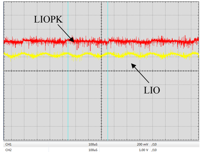
Figure 26. Digital Modulation Response at LIOPK & LIO Pin (f=6kHz)
