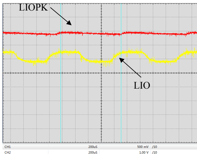
Figure 16. Digital Modulation Response at LIOPK & LIO Pin (f=1kHz)
