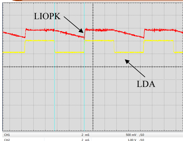
Figure 11. Digital Modulation Response at LIOPK & LDA Pin (f=100Hz)
