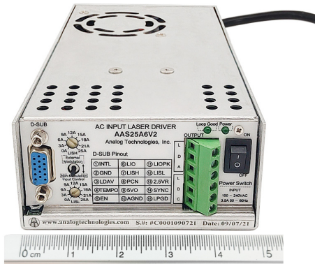
Figure 1. Front View of the AAS25A6V2
