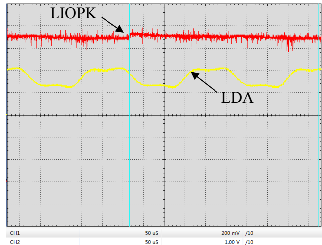
Figure 21. Digital Modulation Response at LIOPK & LDA Pin ( f=4\text{kHz} )
