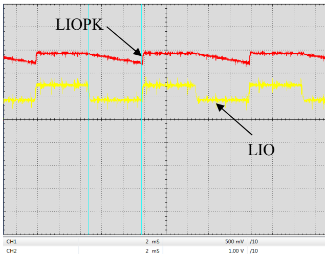
Figure 12. Digital Modulation Response at LIOPK & LIO Pin ( f=100\text{Hz} )
