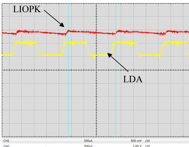
Figure 13. Digital Modulation Response at LIOPK & LDA Pin ( f=500\text{Hz} )
