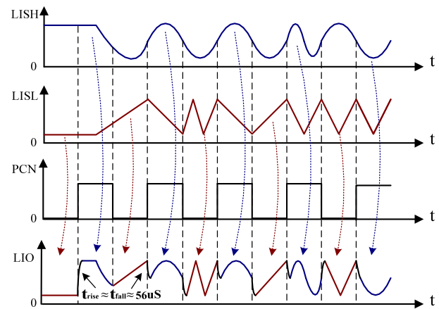
Figure 6. Digitally Controlled Analog Modulation Principle
