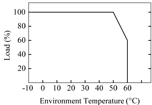
Figure 27. Derating Curve
