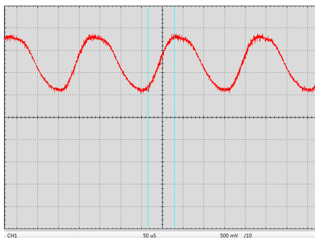
Figure 10. Digital Modulation Response at LDA Pin
