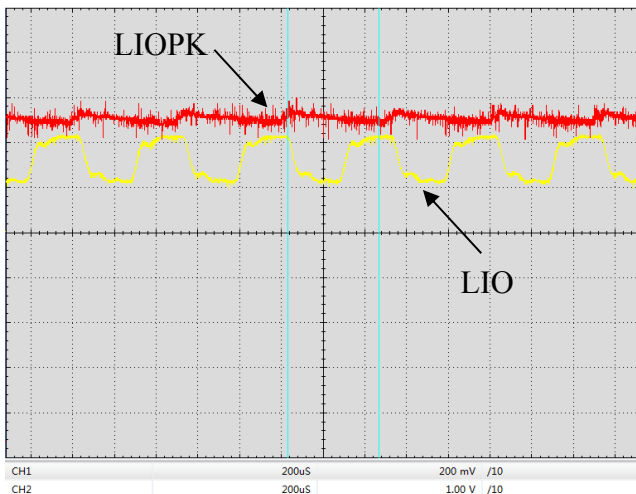
Figure 18. Digital Modulation Response at LIOPK & LIO Pin (f=2kHz)
