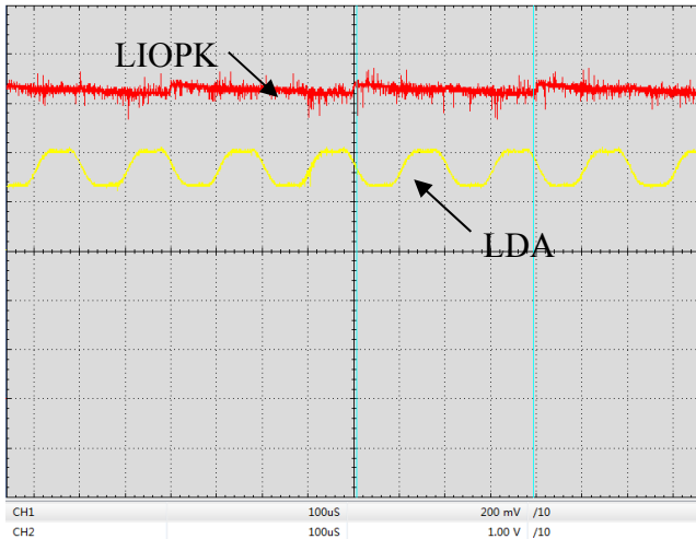
Figure 23. Digital Modulation Response at LIOPK & LDA Pin (f=5kHz)
