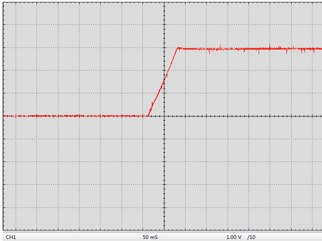
Figure 28. Start-up Waveform at LDA Pin
