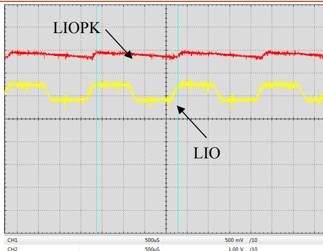
Figure 14. Digital Modulation Response at LIOPK & LIO Pin (f=500Hz)
