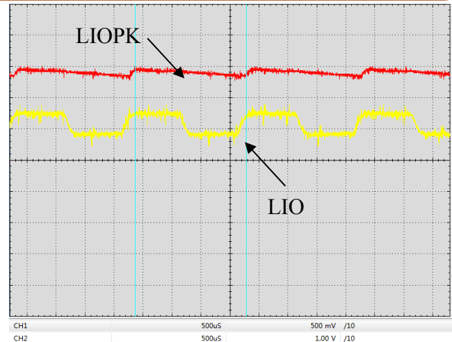
Figure 14. Digital Modulation Response at LIOPK & LIO Pin ( f=500\text{Hz} )
