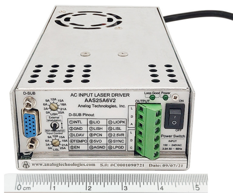
Figure 1. Front View of the AAS25A6V2
