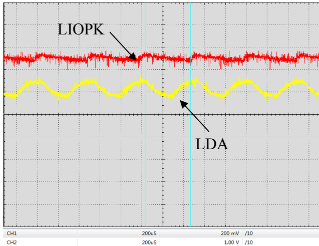
Figure 17. Digital Modulation Response at LIOPK & LDA Pin ( f=2\text{kHz} )
