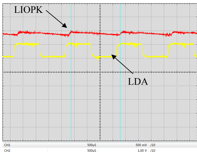
Figure 13. Digital Modulation Response at LIOPK & LDA Pin (f=500Hz)
