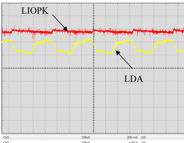
Figure 19. Digital Modulation Response at LIOPK & LDA Pin (f=3kHz)
