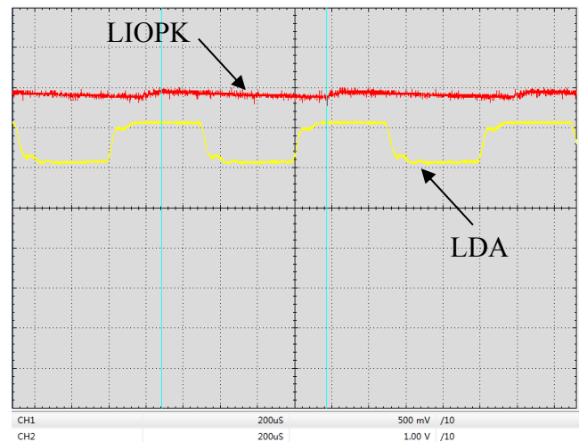
Figure 15. Digital Modulation Response at LIOPK & LDA Pin ( f=1\text{kHz} )
