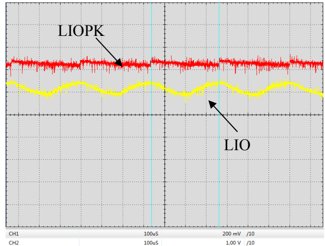
Figure 20. Digital Modulation Response at LIOPK & LIO Pin (f=3kHz)
