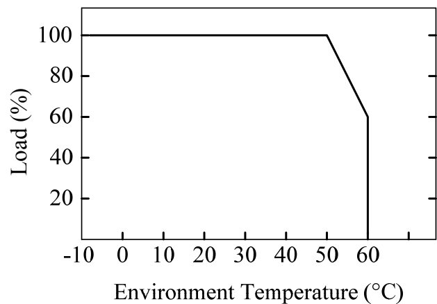
Figure 27. Derating Curve
