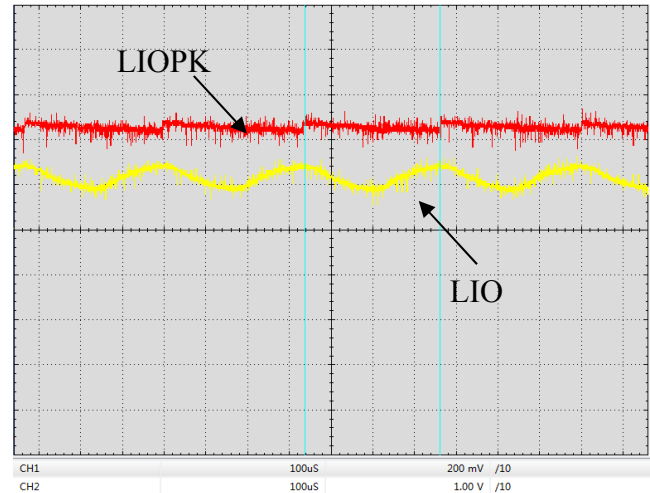
Figure 20. Digital Modulation Response at LIOPK & LIO Pin ( f=3\text{kHz} )
