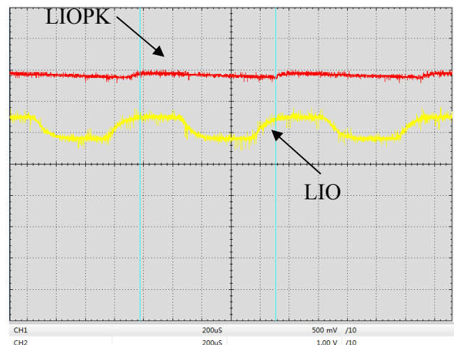
Figure 16. Digital Modulation Response at LIOPK & LIO Pin ( f=1\text{kHz} )
