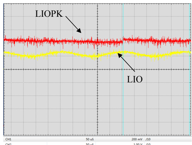
Figure 22. Digital Modulation Response at LIOPK & LIO Pin (f=4kHz)
