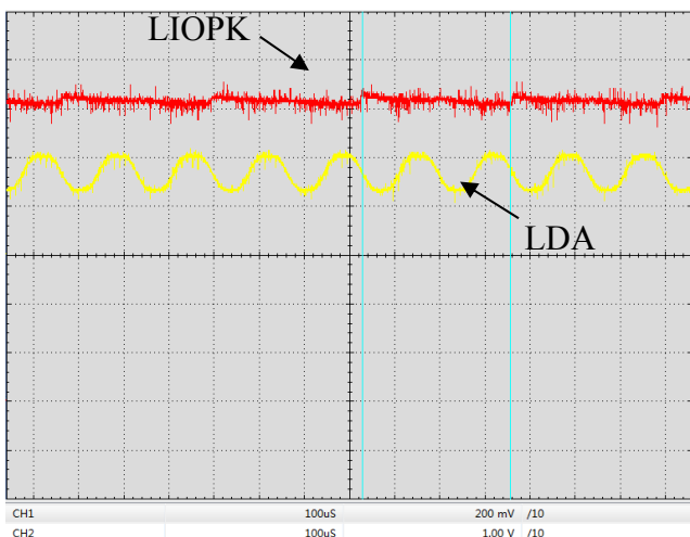
Figure 25. Digital Modulation Response at LIOPK & LDA Pin (f=6kHz)
