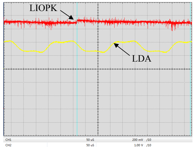
Figure 21. Digital Modulation Response at LIOPK & LDA Pin (f=4kHz)
