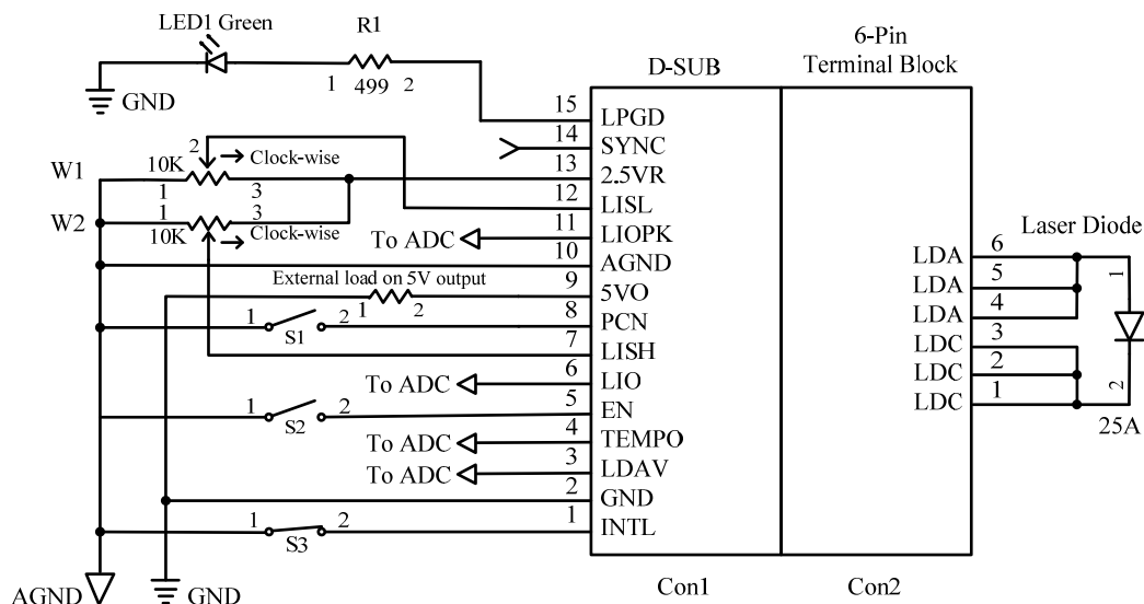
Figure 5. A Typical Application Schematic
