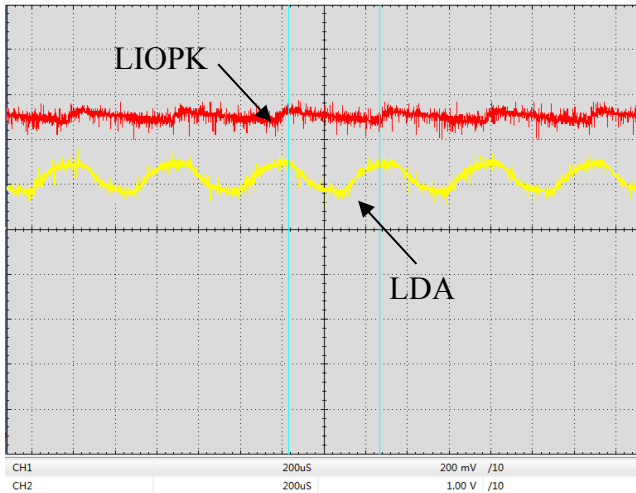
Figure 17. Digital Modulation Response at LIOPK & LDA Pin (f=2kHz)
