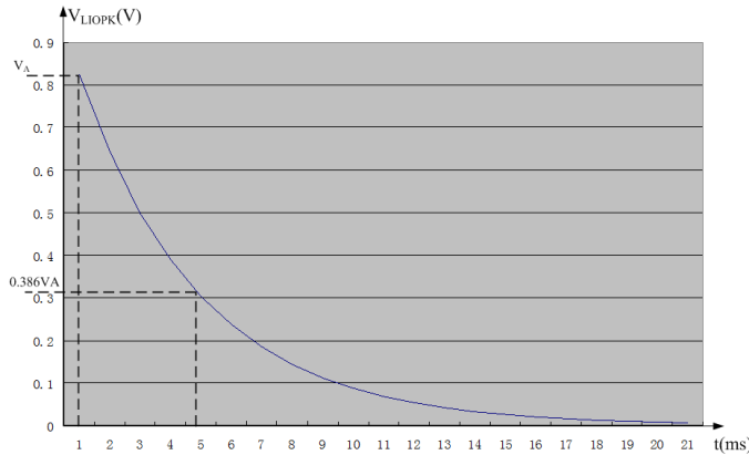
Figure 7. LIOPK's Mathematic Model
