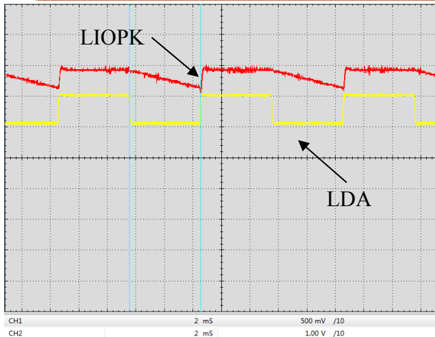
Figure 11. Digital Modulation Response at LIOPK & LDA Pin ( f=100\text{Hz} )
