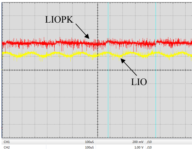
Figure 24. Digital Modulation Response at LIOPK & LIO Pin (f=5kHz)
