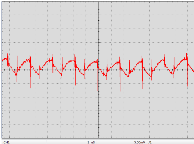
Figure 29. Noise Waveform at LDA Pin
