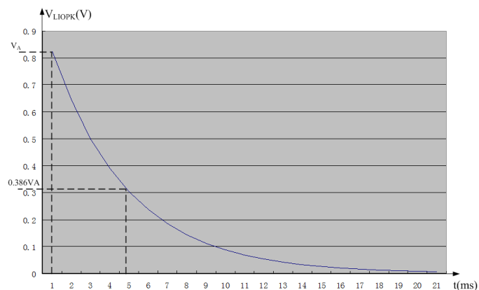
Figure 7. LIOPK's Mathematic Model
