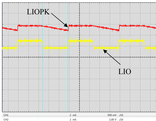
Figure 12. Digital Modulation Response at LIOPK & LIO Pin (f=100Hz)
