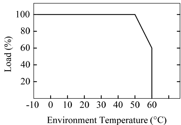
Figure 26. Derating Curve
