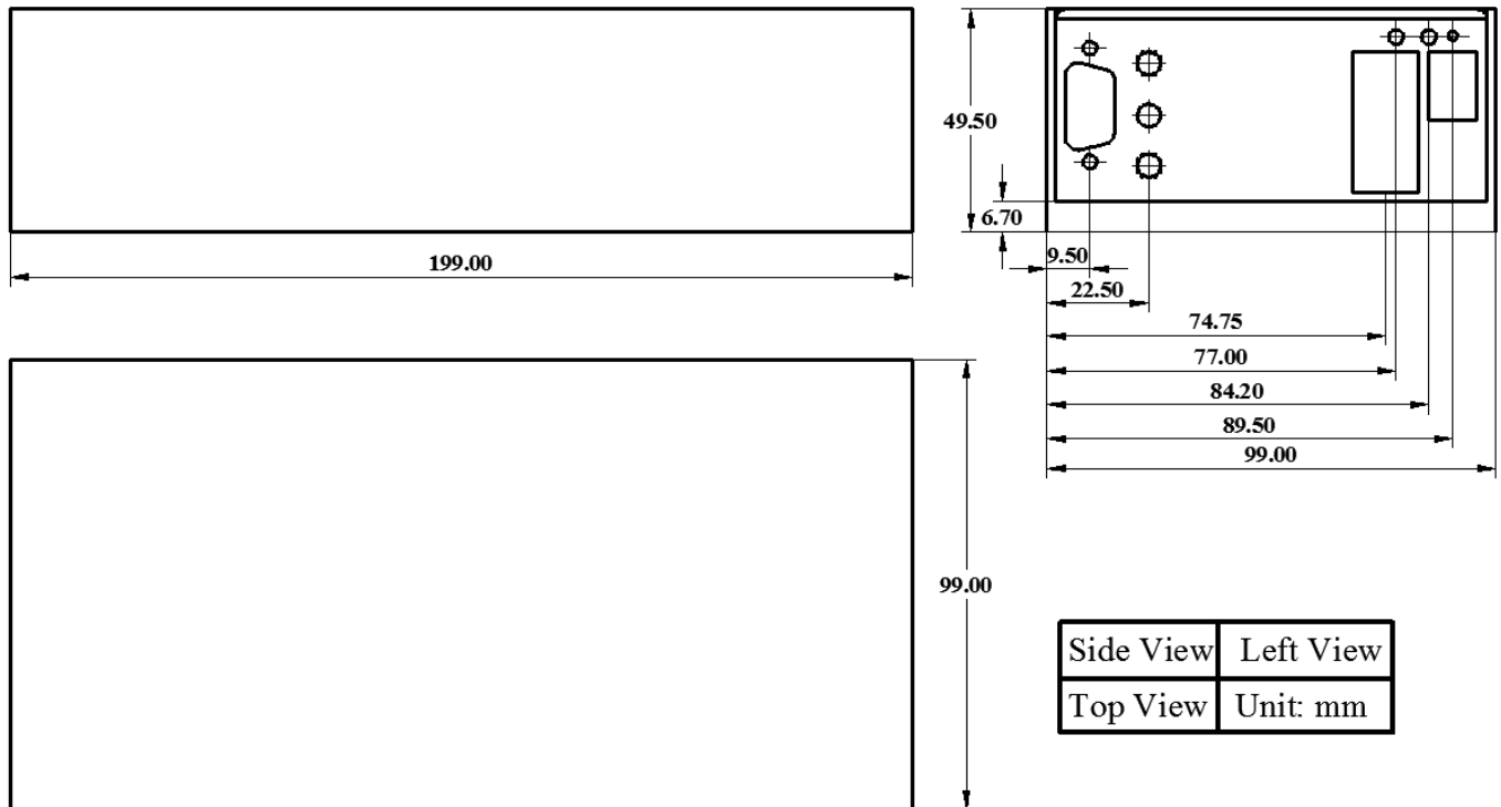
Figure 29. Mechanical Dimensions
