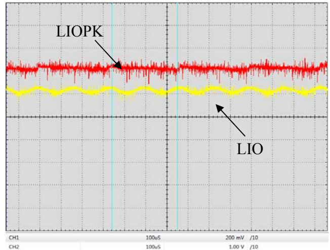
Figure 25. Digital Modulation Response at LIOPK & LIO Pin (f=6kHz)
