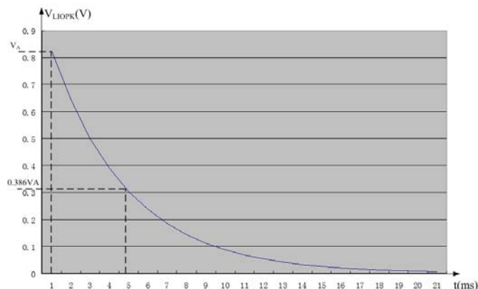
Figure 6. LIOPK's Mathematic Model
