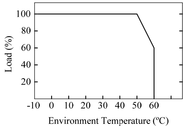
Figure 16. Derating Curve
