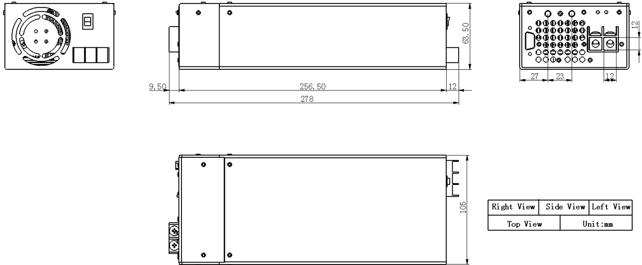
Figure 19. Mechanical Dimensions
