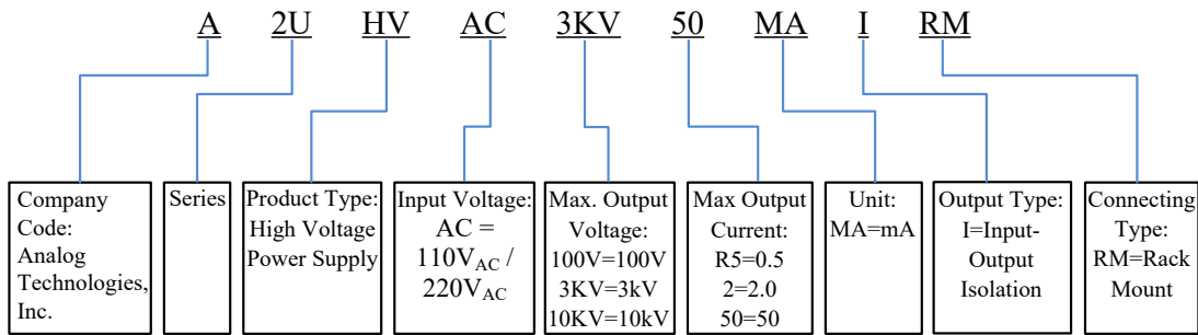
Figure 8. Naming Rules of A2UHVAC3KV50MAIRM
