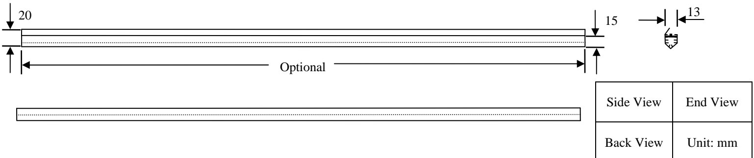
Figure 6. Mechanical Dimensions(2)
