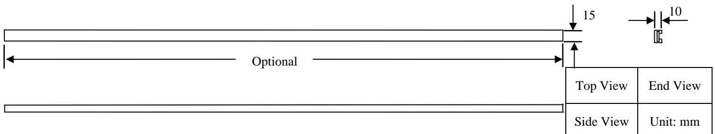
Figure 5. Mechanical Dimensions(1)
