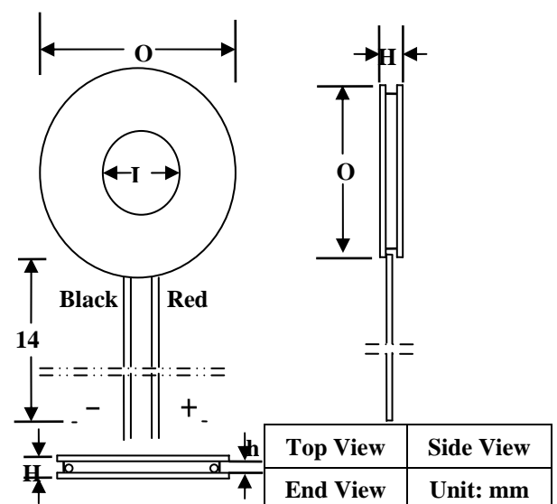
Figure 3. Mechanical dimensions of ATE1-38-3.4A
