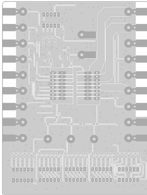
Figure 4. Top Layers without Top Screen Layer
