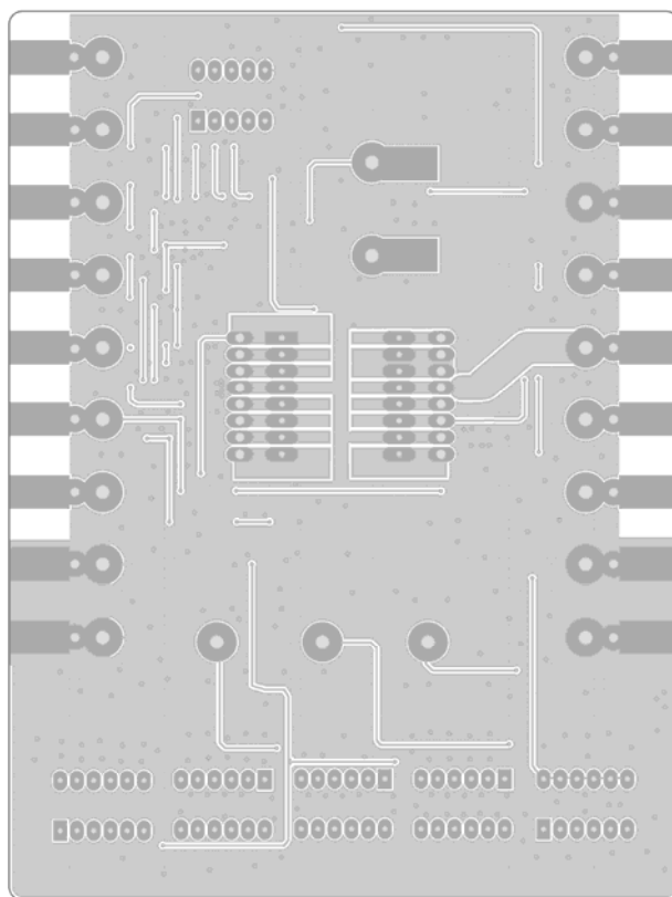
Figure 5. Bottom Layers
