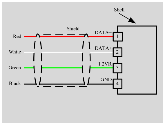
Figure 3. Connecting DAC Board to the QCL Driver AQCL1A410DF
