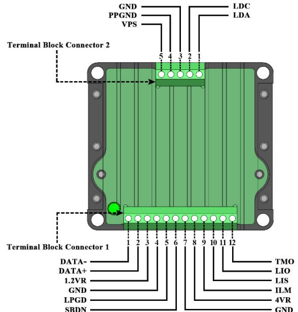
Figure 4. Top View of AQCL1A410DF
