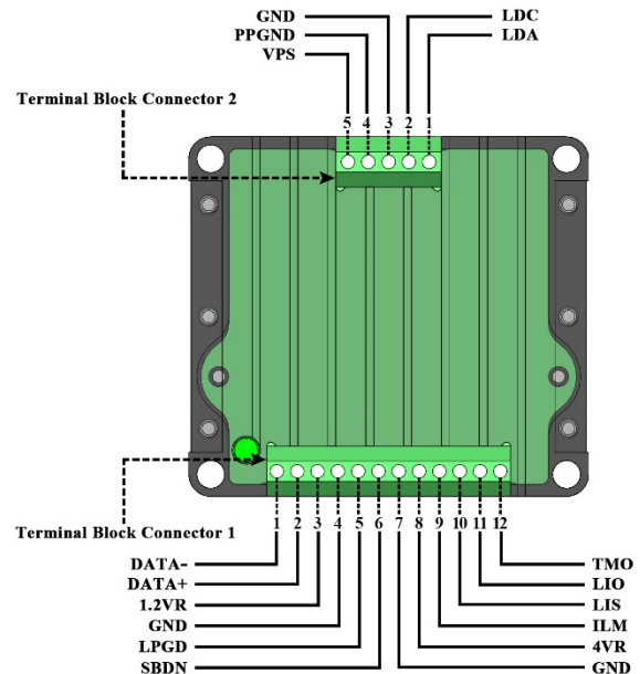
Figure 4. Top View of AQCL100MA410DF
