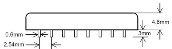
Figure 8. Side View of LDA1-CP1-D
