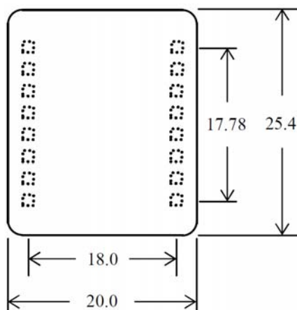
Figure 7. Top View of LDA1-CP1-D
