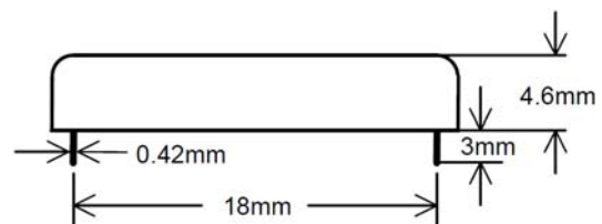
Figure 9. End View of LDA1-CP1-D
