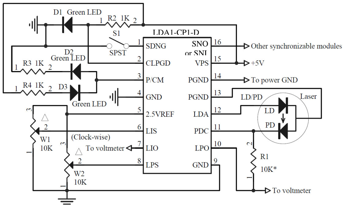
Figure 5. A Typical Self-contained Application Schematic
