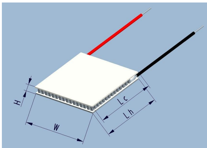
Single stage TEC Module (Non-sealed)
