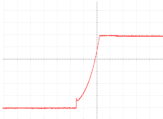
The soft start of startup by both power supply and the switch. When the current is 0.03A, the voltage is 6V.
