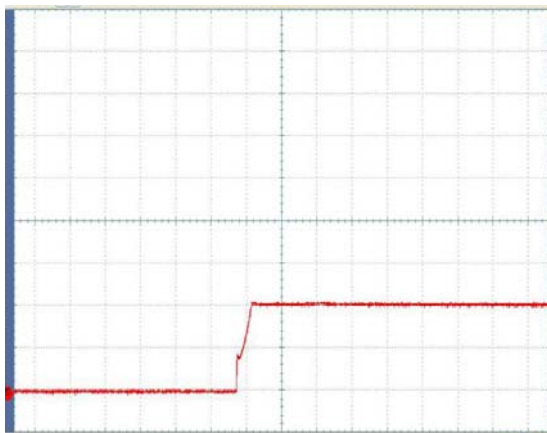
The soft start of startup by both power supply and the switch. When the current is 0.03A, the voltage is 2V.
