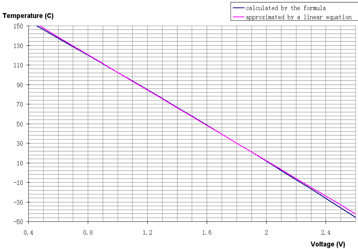
Figure 7. Controller Internal Temperature vs. TMPO Voltage
