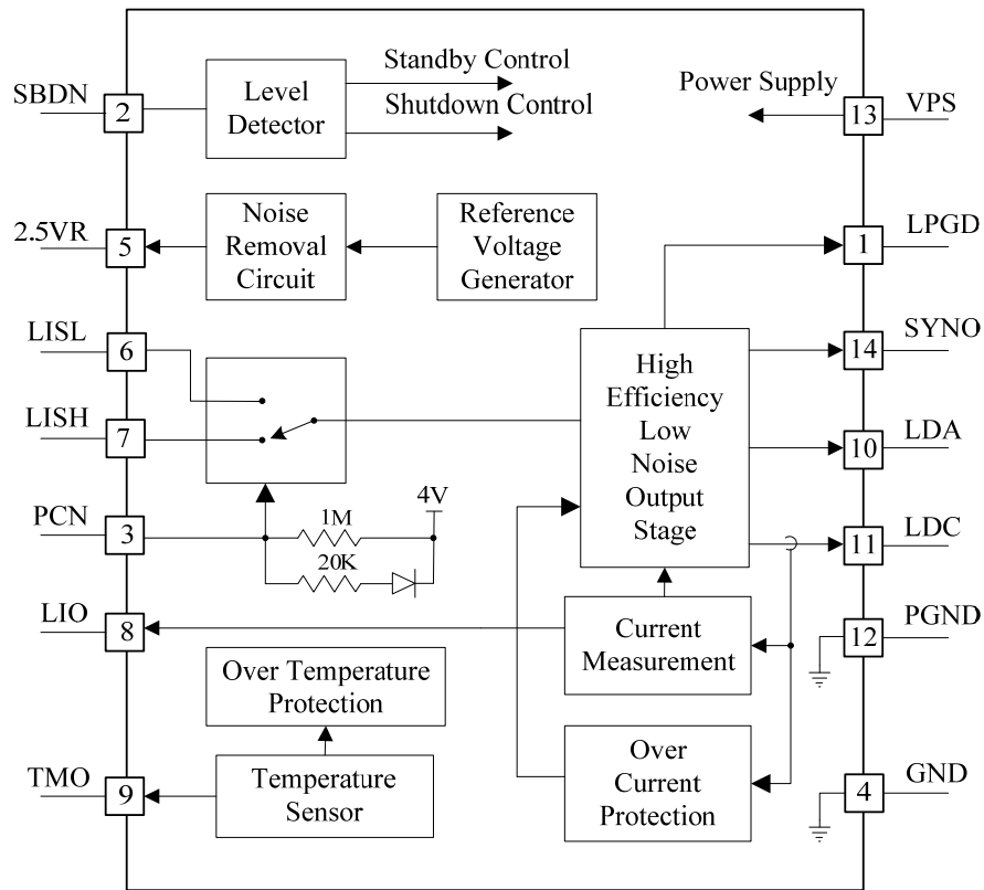
Figure 3. Internal Block Diagram of ATLS50MA212
