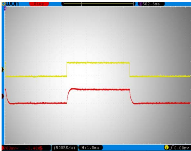
Figure 13. Small Signal Modulation
