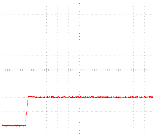
The soft start of startup by both power supply and the switch. When the current is 0.05A, the voltage is 2V.
