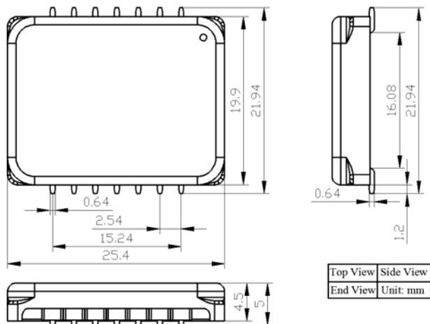
Figure 15. Dimensions of the SMT Package Driver
