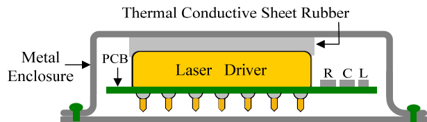
Figure 11. Transferring heat by the gap filler
